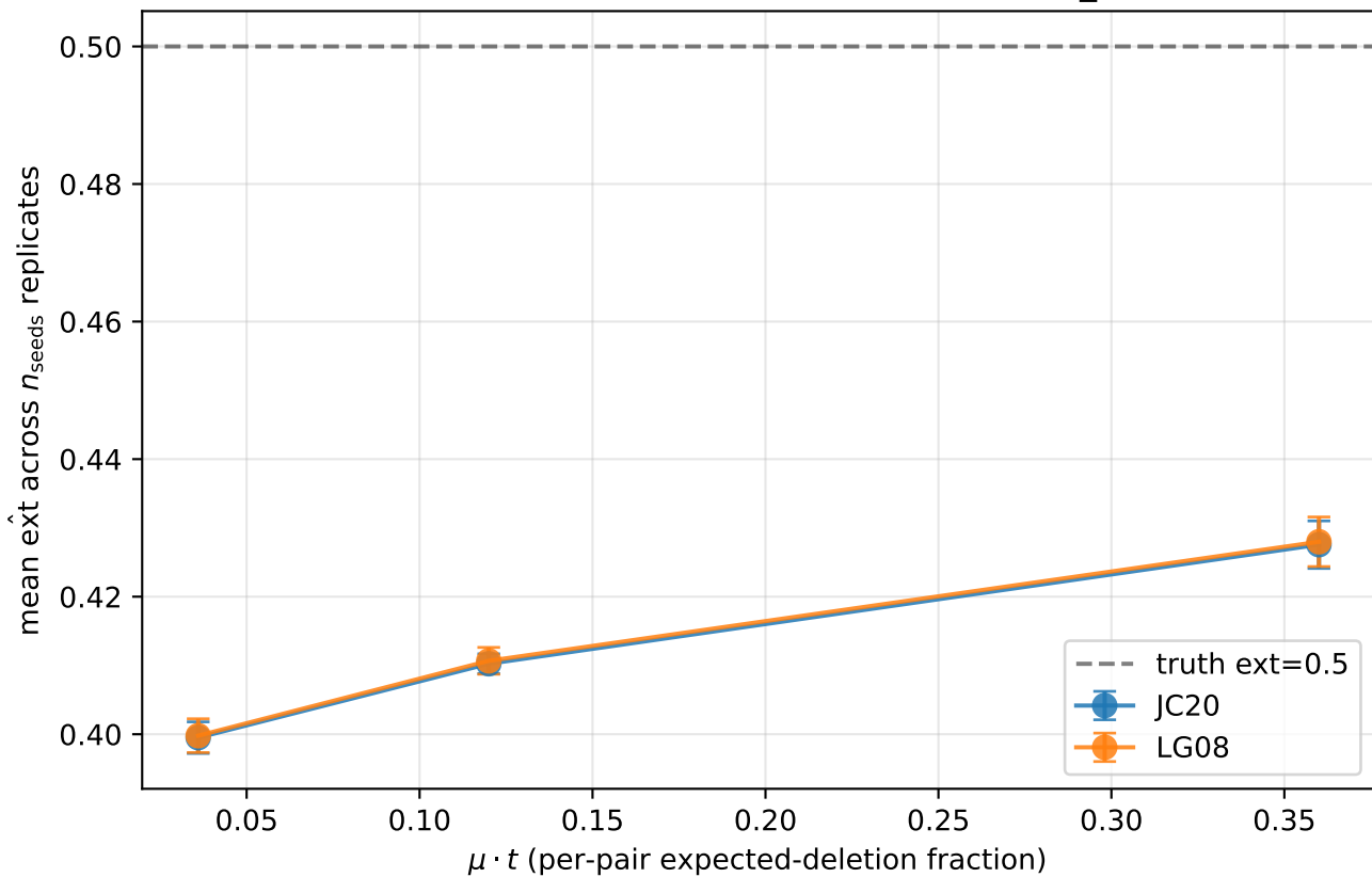
TKF92 ext recovery vs ( t , Q model) ( \text{lam}=0.08 , \mu=0.12 , truth ext=0.5, N=1000 , n_{\text{seeds}}=4 )
