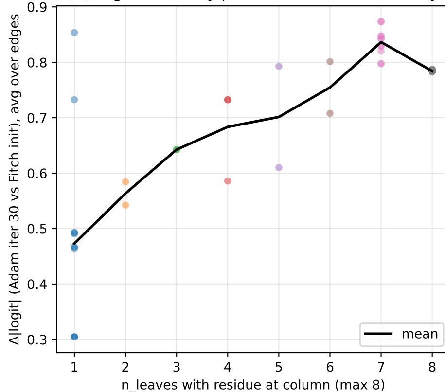
(2) Logit motion by per-column data availability
