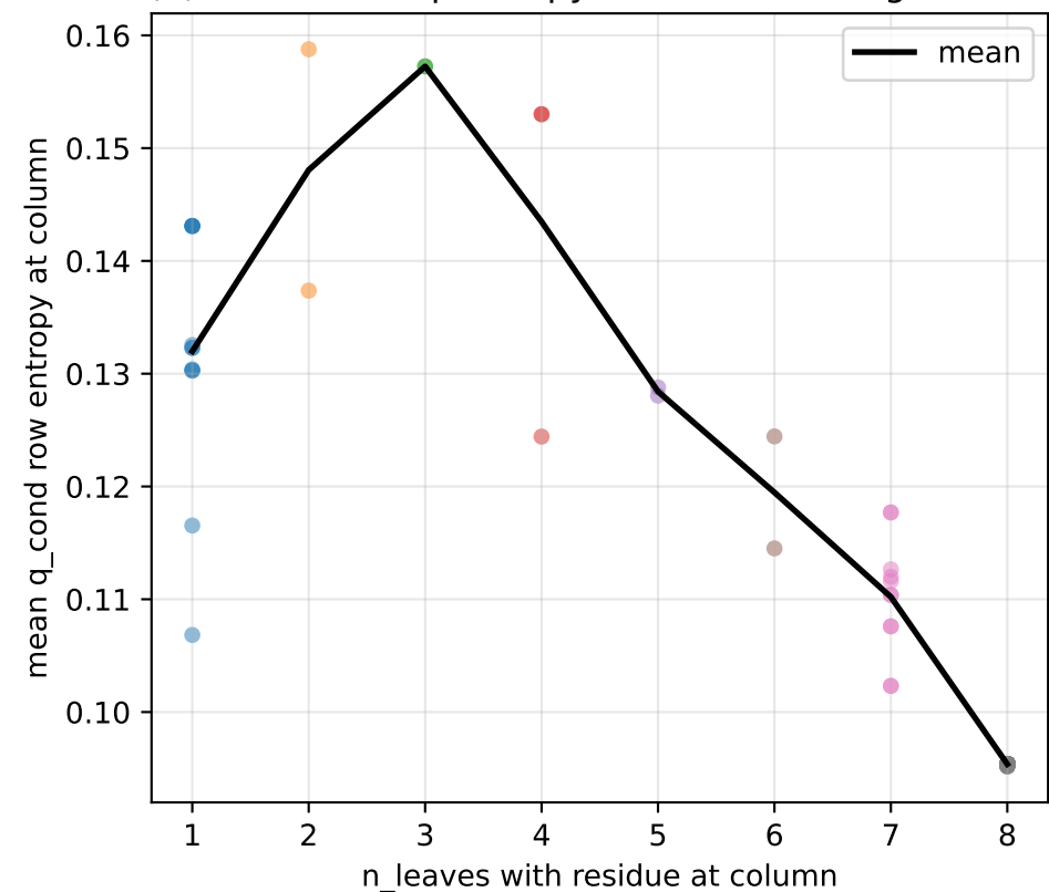
(3) Per-column q-entropy at Adam-converged state
