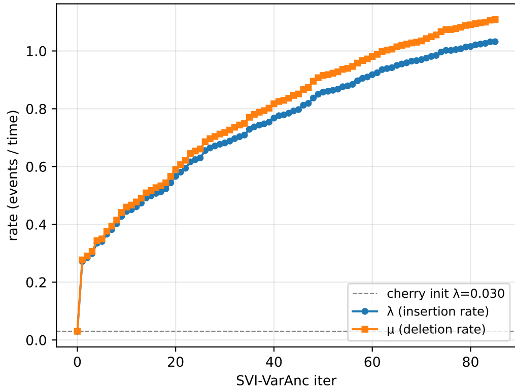
(A) Real Pfam: 19{,}850 train families (checkpoint at iter 85)
