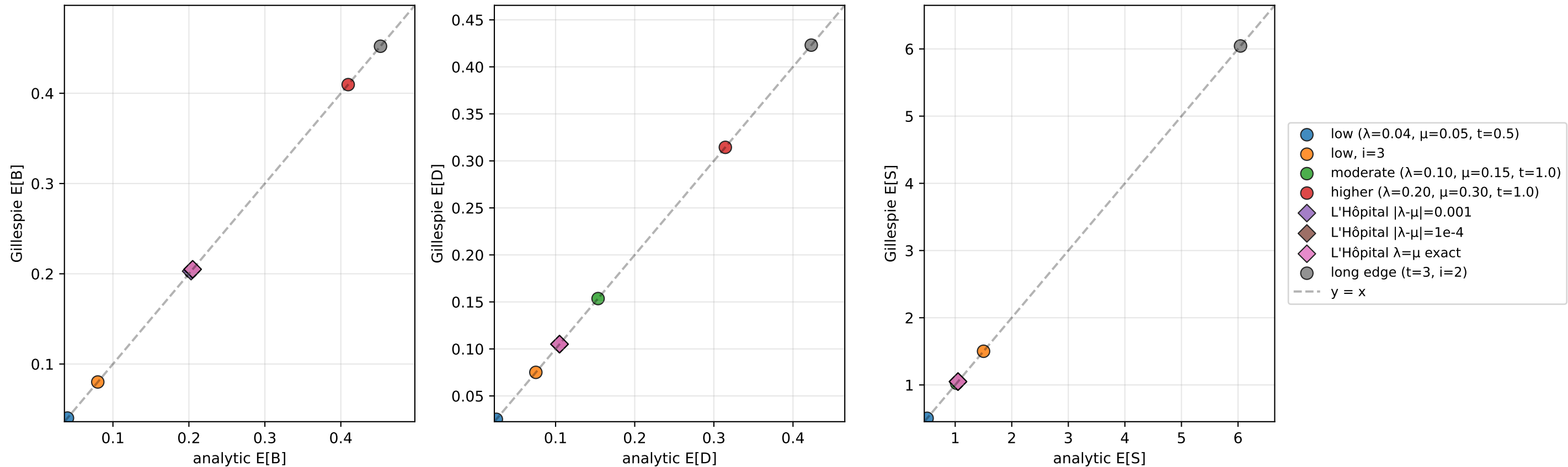
TKF BDI Gillespie vs analytic moments ( n_{\text{sims}} = 20000000 ). Diamonds: L'Hôpital regime ( \lambda \approx \mu ).
