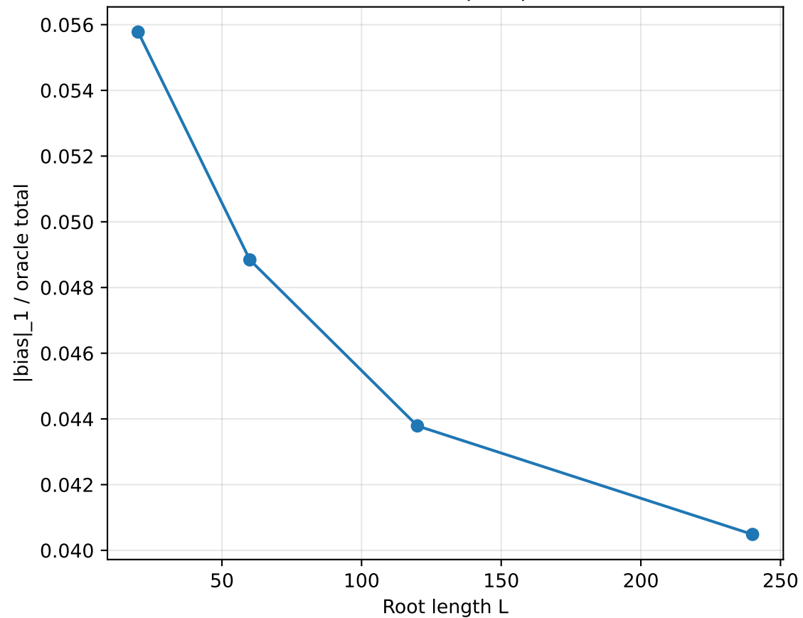
(A) Relative bias |bias| / oracle
