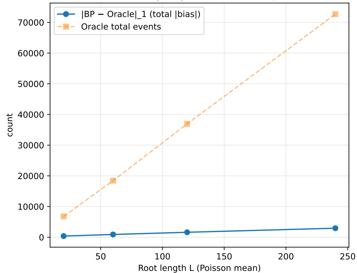
(A) Total |bias| vs root chain length
