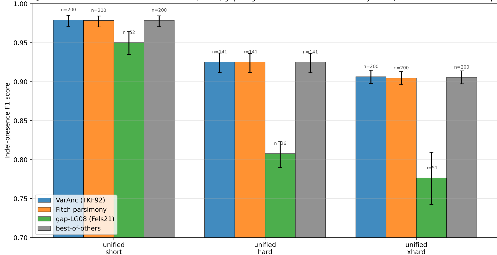
TKF §5: ancestral indel reconstruction. VarAnc, Fitch, gap-augmented LG08 across difficulty tiers (error bars: 95% bootstrap CI).
