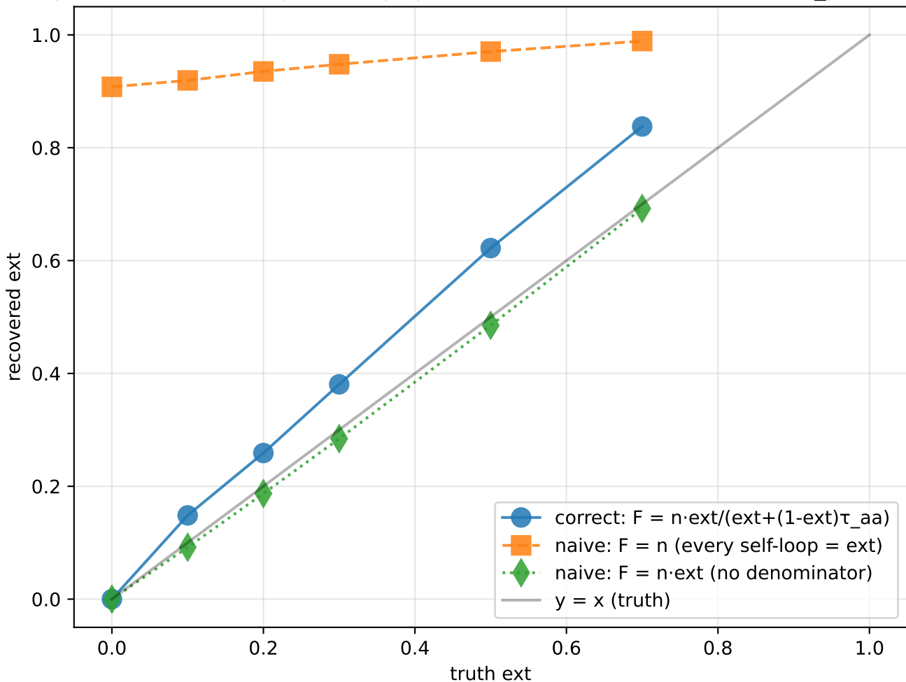
Fragment-extension responsibility split: correct vs naive alternatives (n_pairs=2000)
