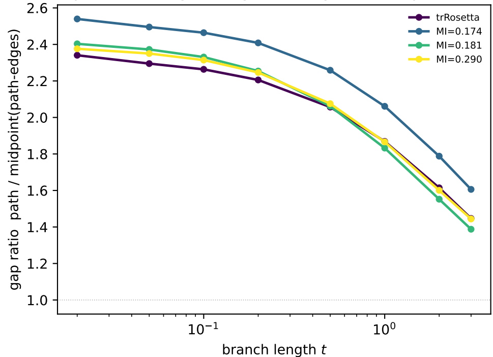
Midpoint-node tightening ( >1 = tighter than path ELBO)
