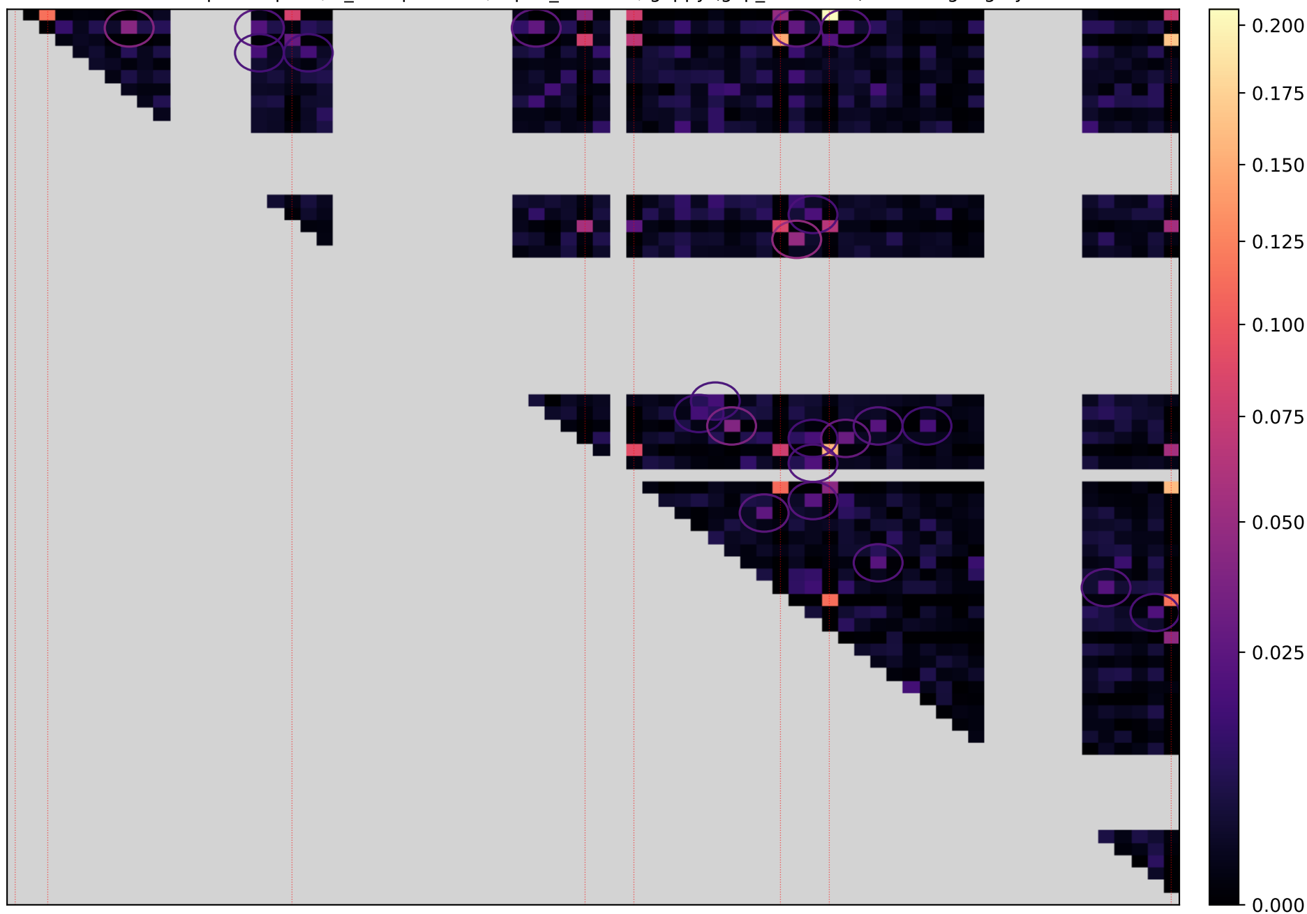
Composite-likelihood edge-pair posterior over MSA columns: PF00053 (Laminin EGF-like) 8 sequence-pairs, n_sweeps=1500, alpha_z=100.0; gappy (gap_frac > 0.5) shown light grey
