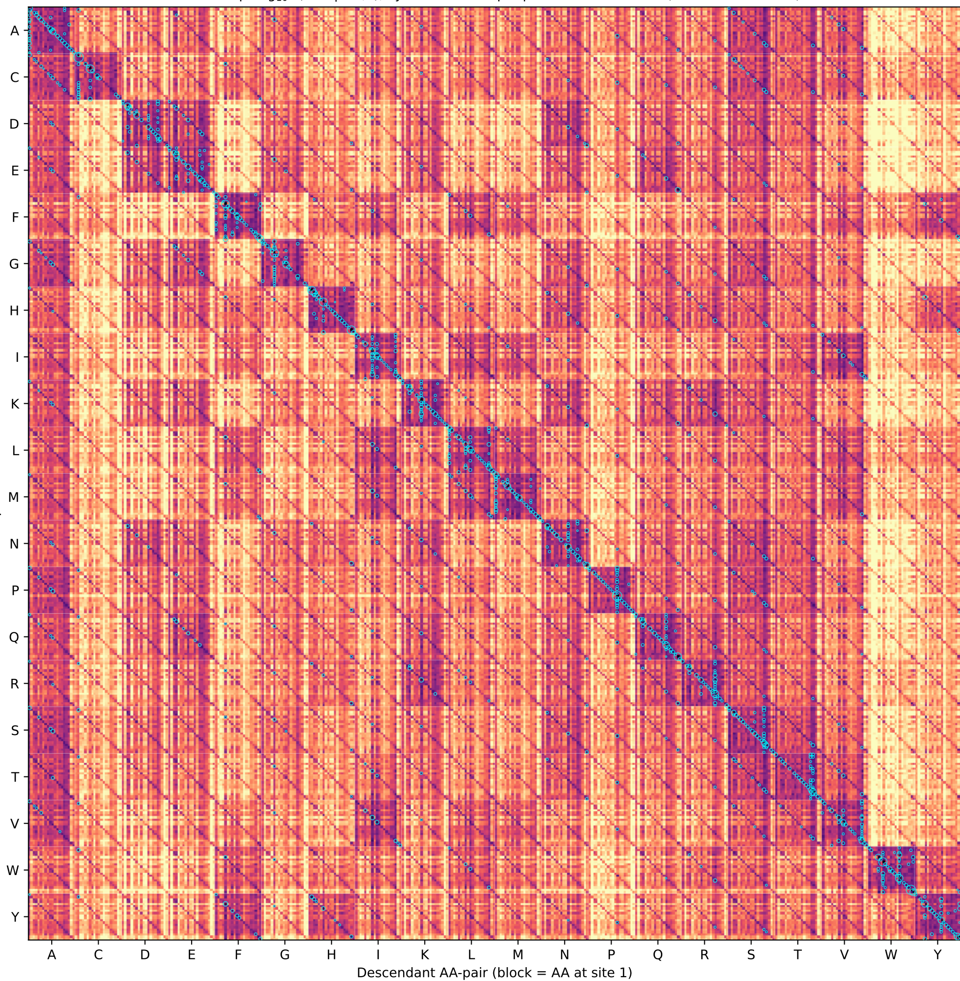
K=4 effective doublet substitution matrix at t = 1.0 (canonical: LG08 pair bg, empirical \pi_c ) heatmap: \log_{10} P(\text{desc}|\text{anc}; t) ; cyan bubbles: top-3 per row with P \geq 0.02 (total 1196 bubbles)
