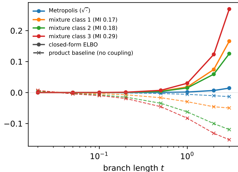
Approximation gap (ELBO is a lower bound)
