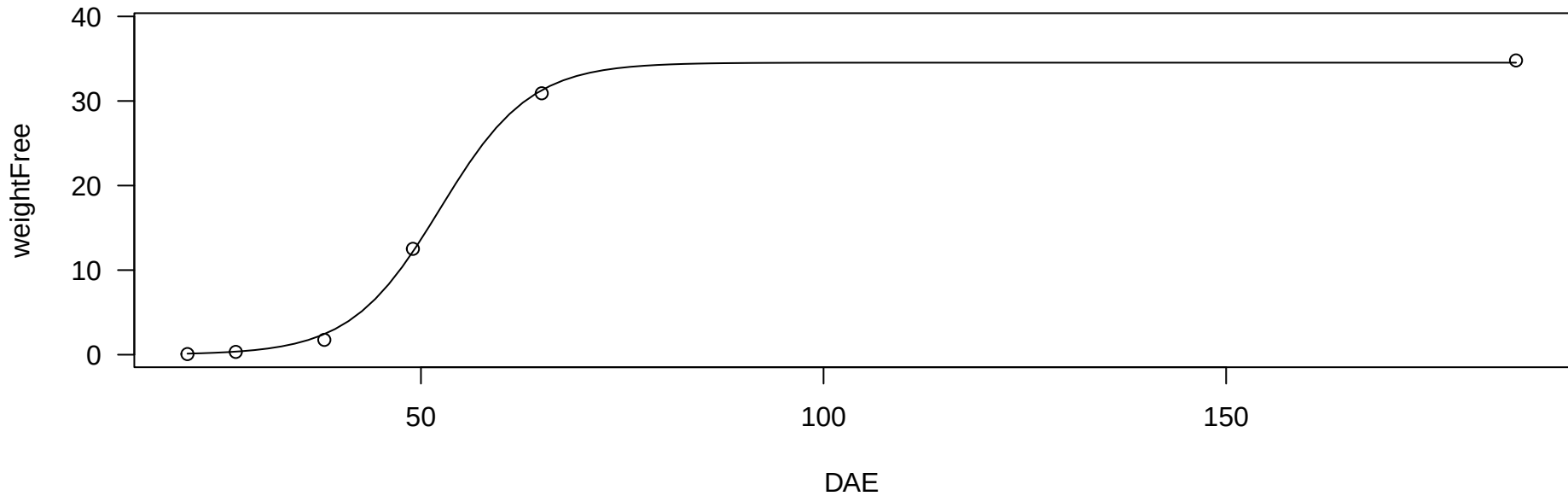
Logistic function
