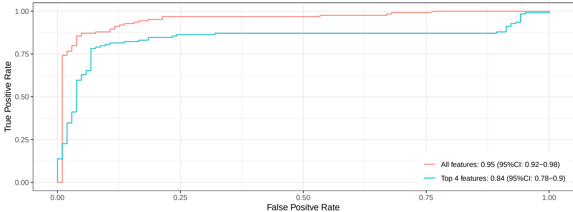
ROC plot
