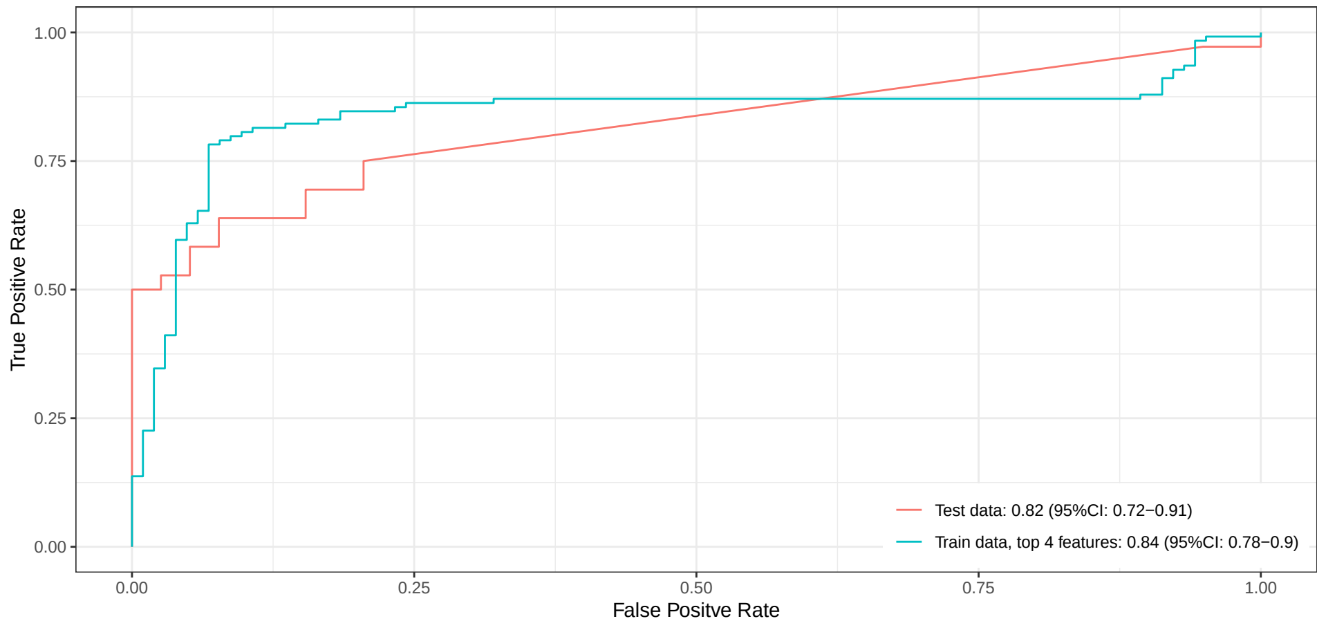
ROC plot
