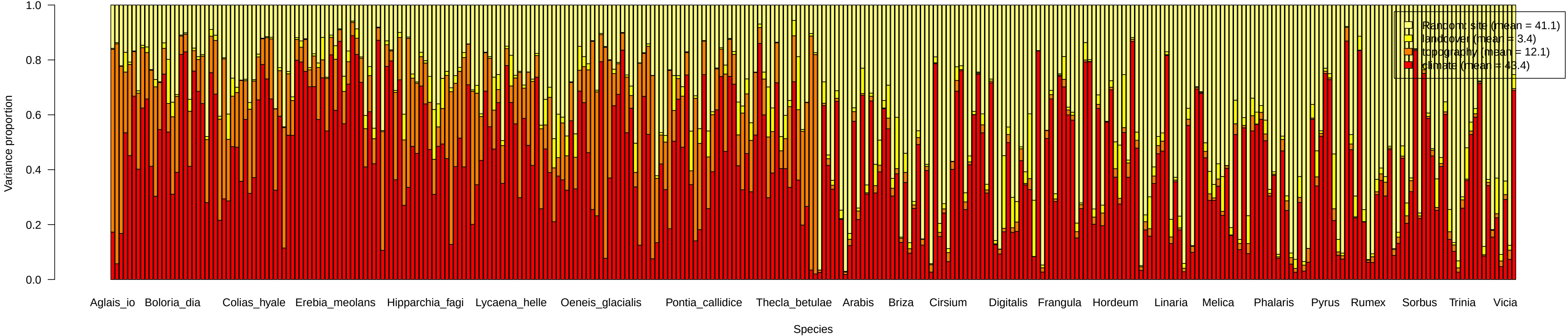
Variance Partitioning
