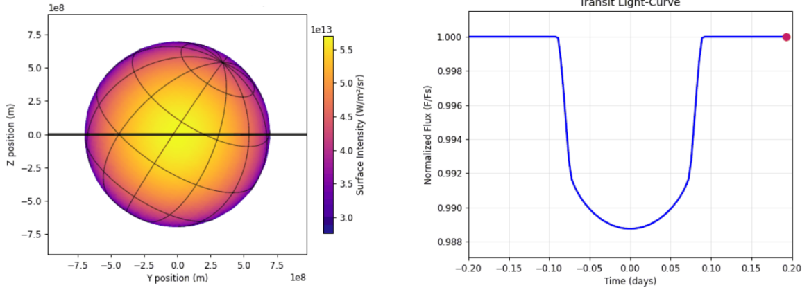
(a) Simulated transit light-curve with \beta = 0.15 , \omega = 0 .
