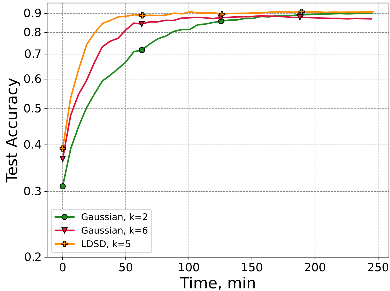
ZO-SGD
