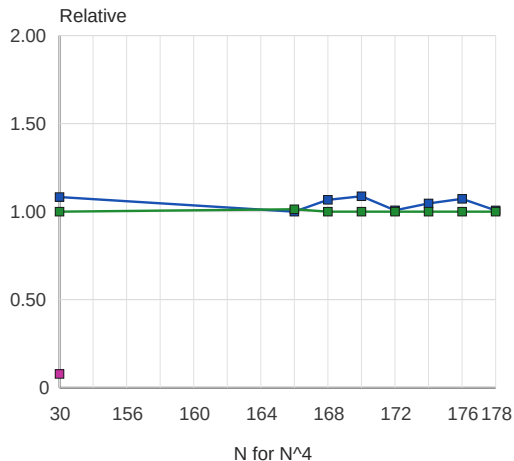
Relative runtime
