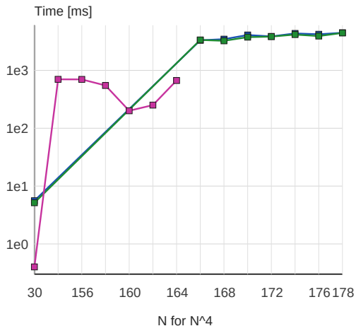
Absolute runtime
