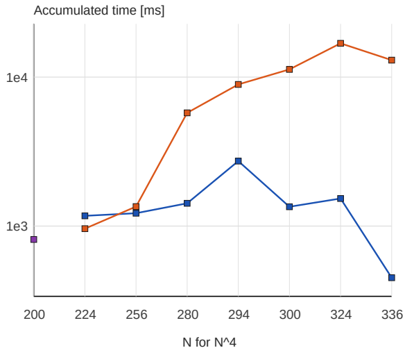
Forward transform
