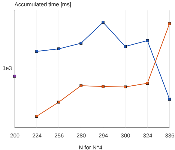
Backward transform
