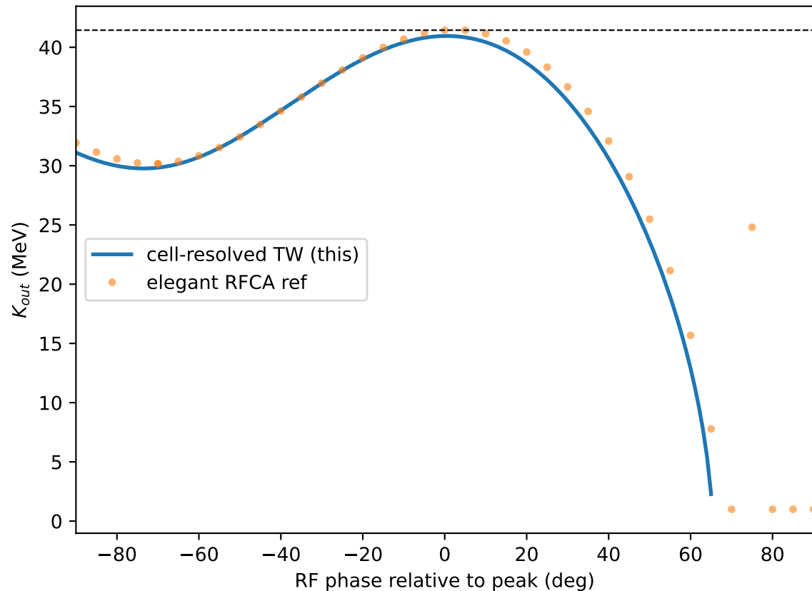
Energy gain vs RF phase, 1 MeV injection
