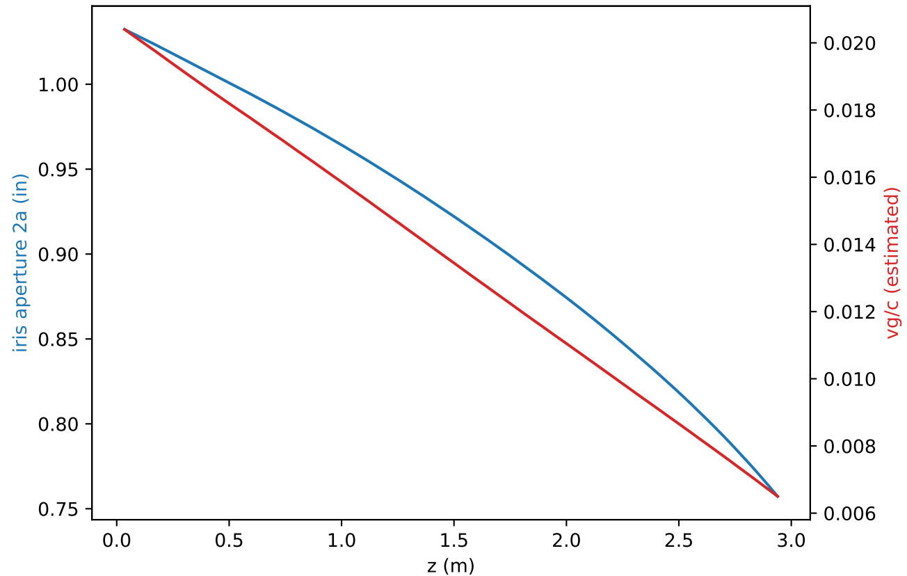
Constant-gradient cell geometry (SLAC-75 Table 6-6)
