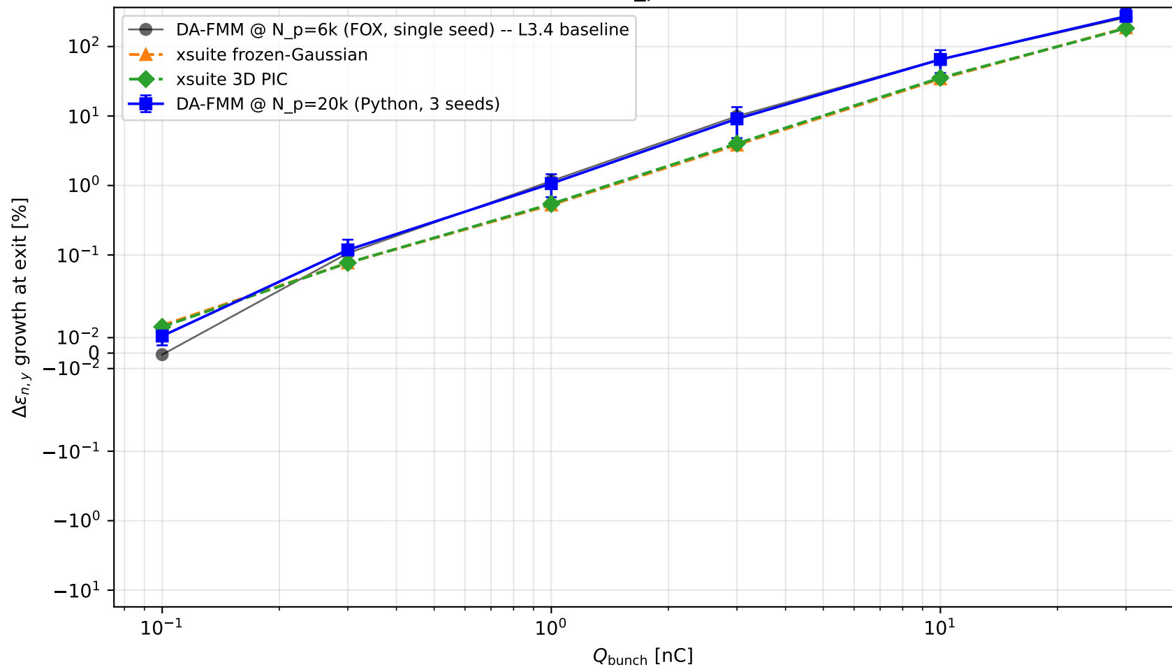
L3.7 item A: DA-FMM at N_p=20k vs xsuite reference
