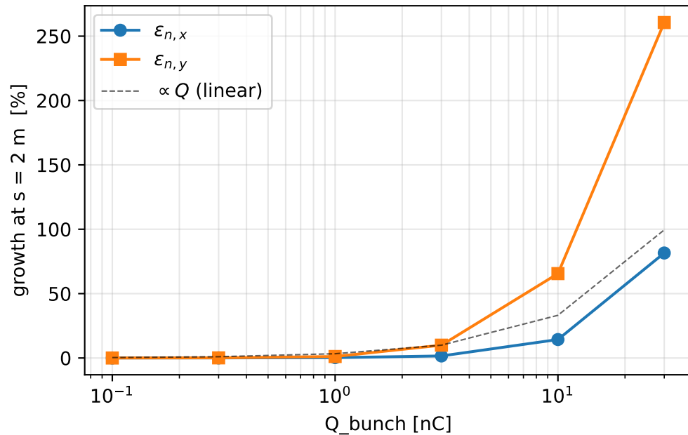
Normalised emittance growth
