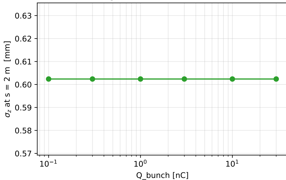
Longitudinal beam size at exit
