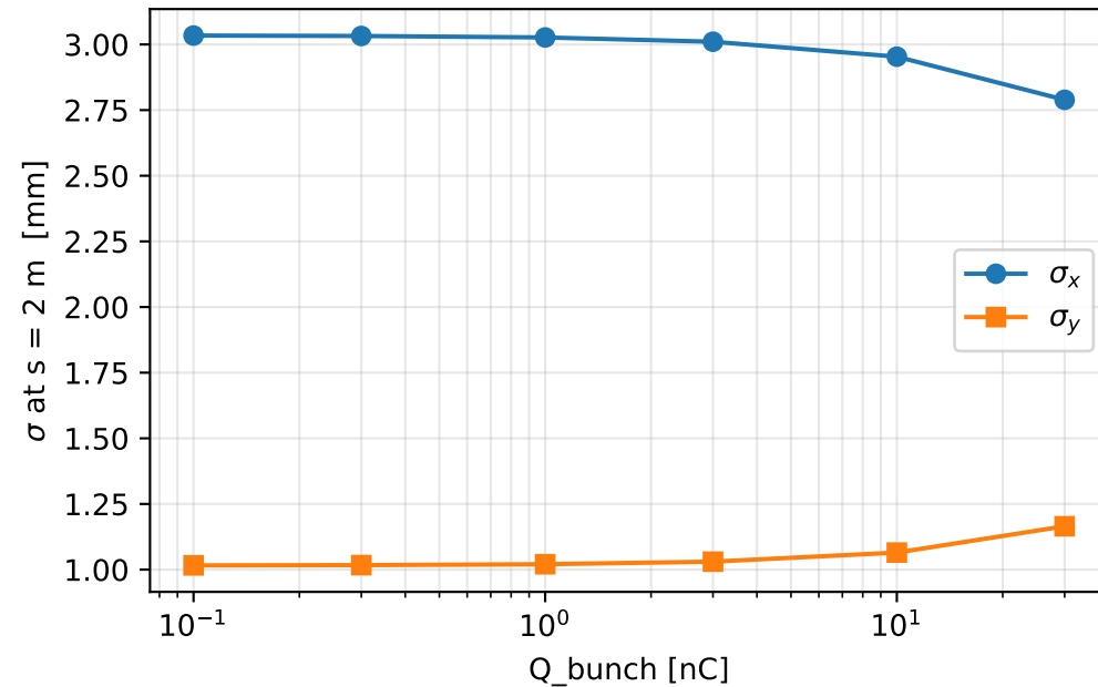
Transverse beam size at exit
