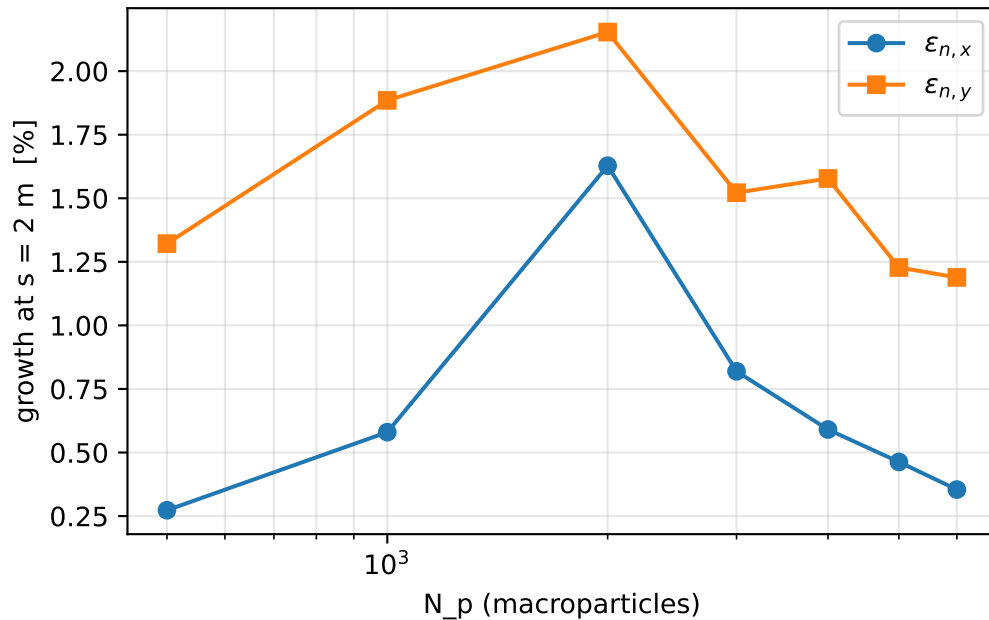
Normalised emittance growth
