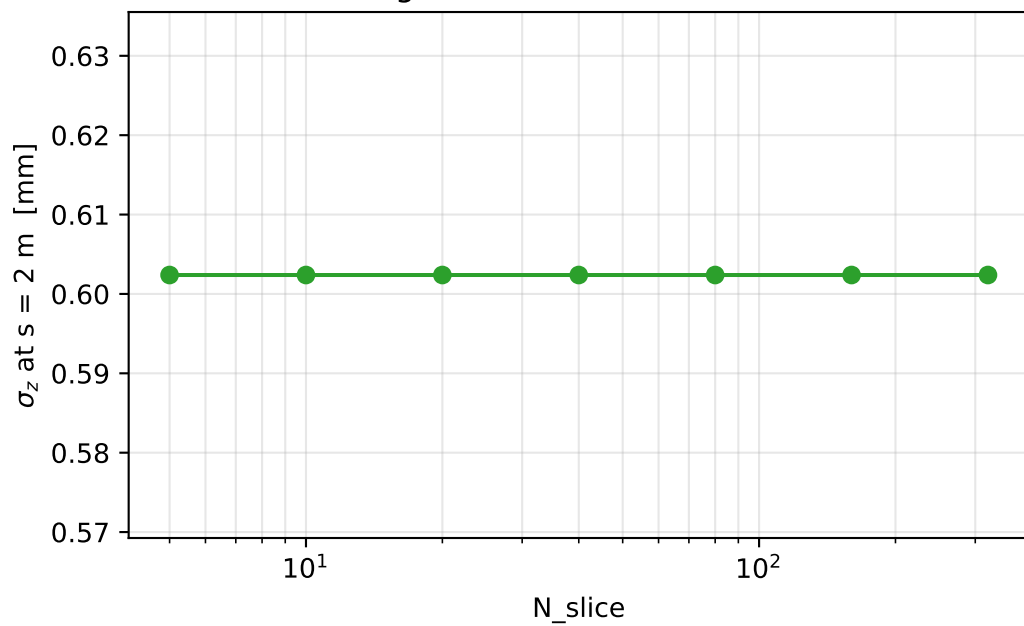
Longitudinal beam size at exit
