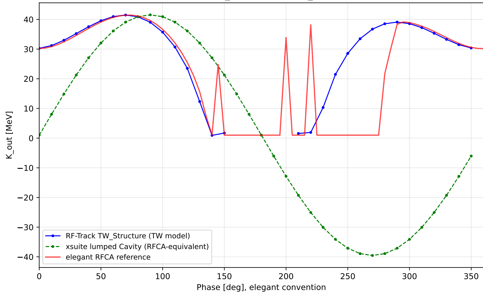
SLAC 3-m TW Linac single-particle phase scan f=2.856 GHz, E_0=13.3 MV/m, K_{inj}=1.0 MeV
