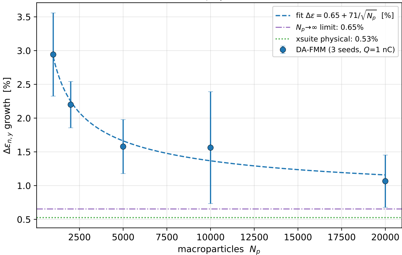
DA-FMM shot noise \sim 1/\sqrt{N_p} converges to physical SC
