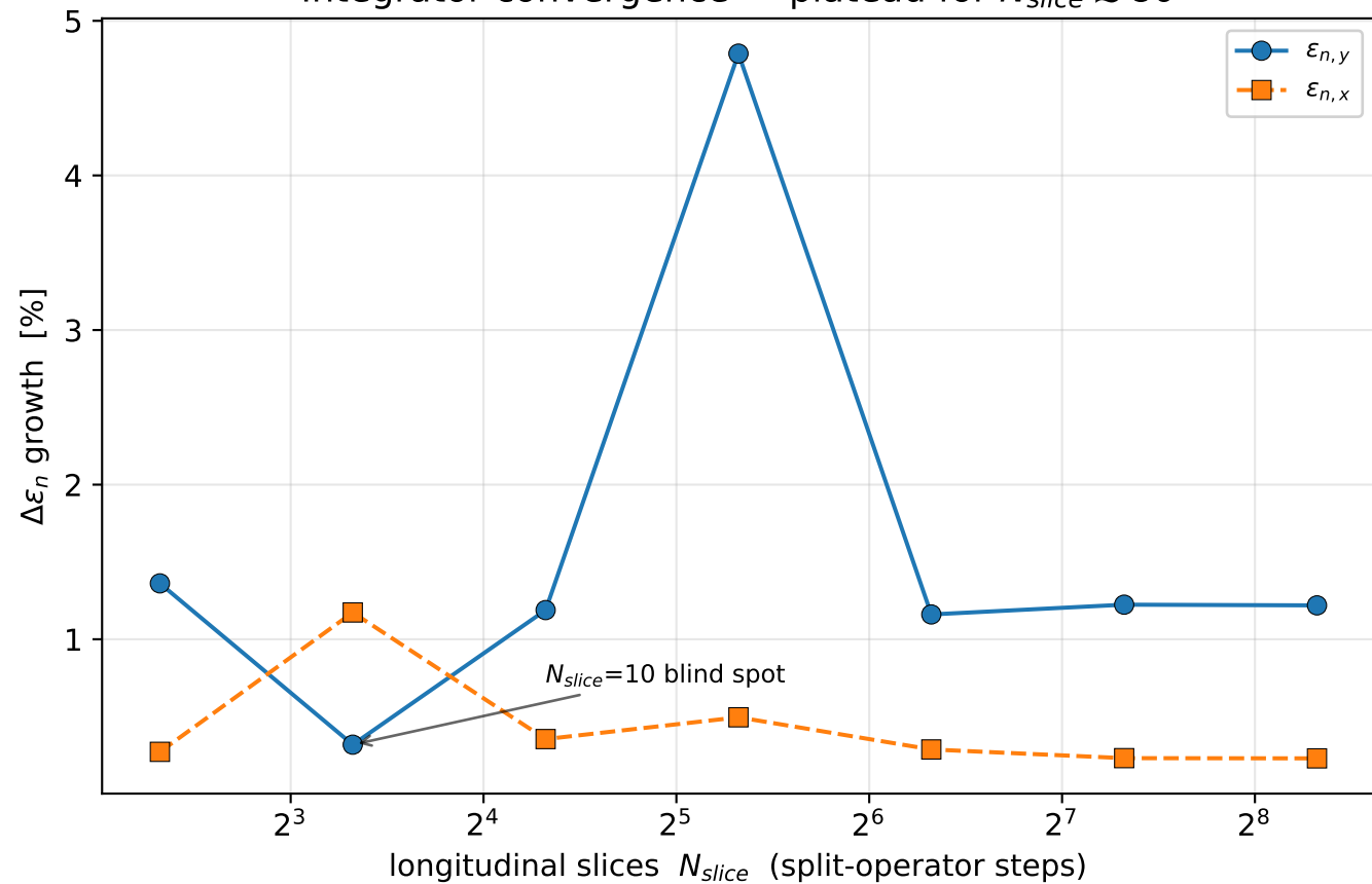
Integrator convergence — plateau for N_{\text{slice}} \gtrsim 80
