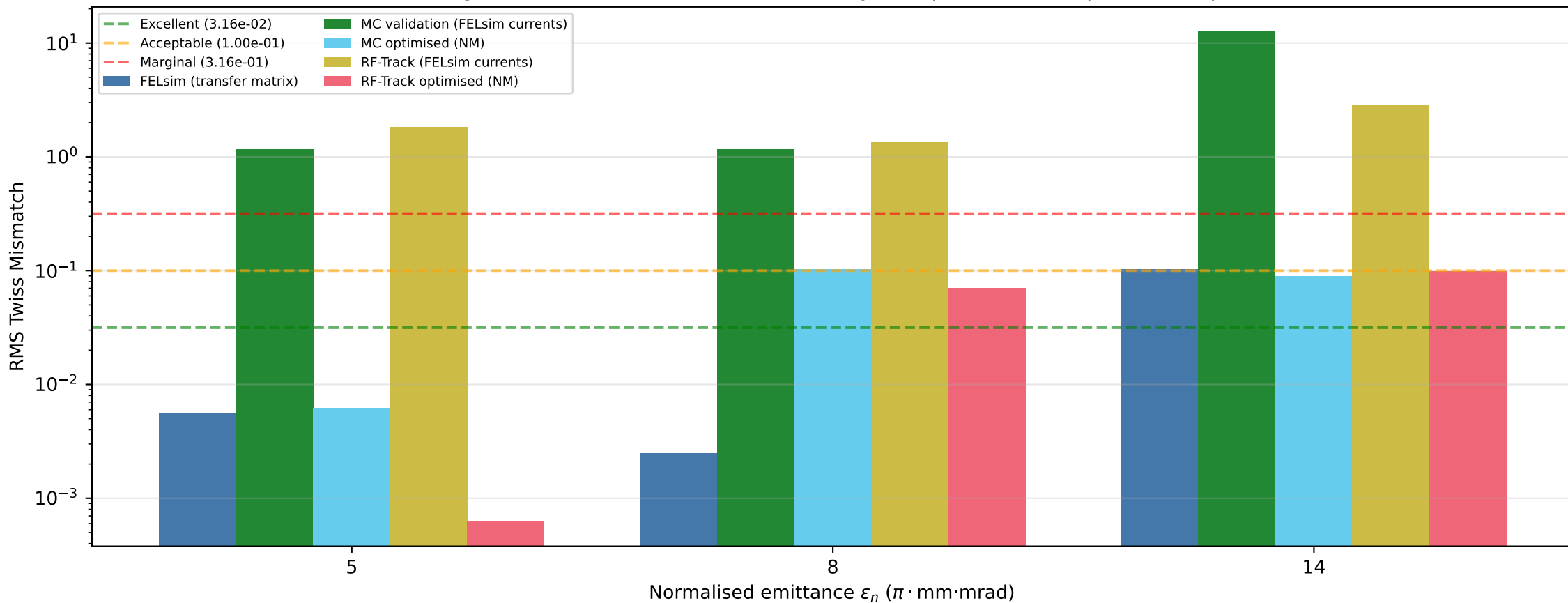
Stage 11 RMS Twiss Mismatch: Five-Way Comparison (MC-opt vs RFT-opt)
