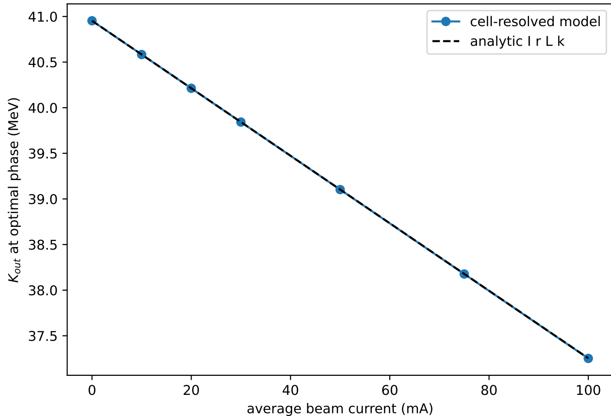
Energy droop vs beam loading
