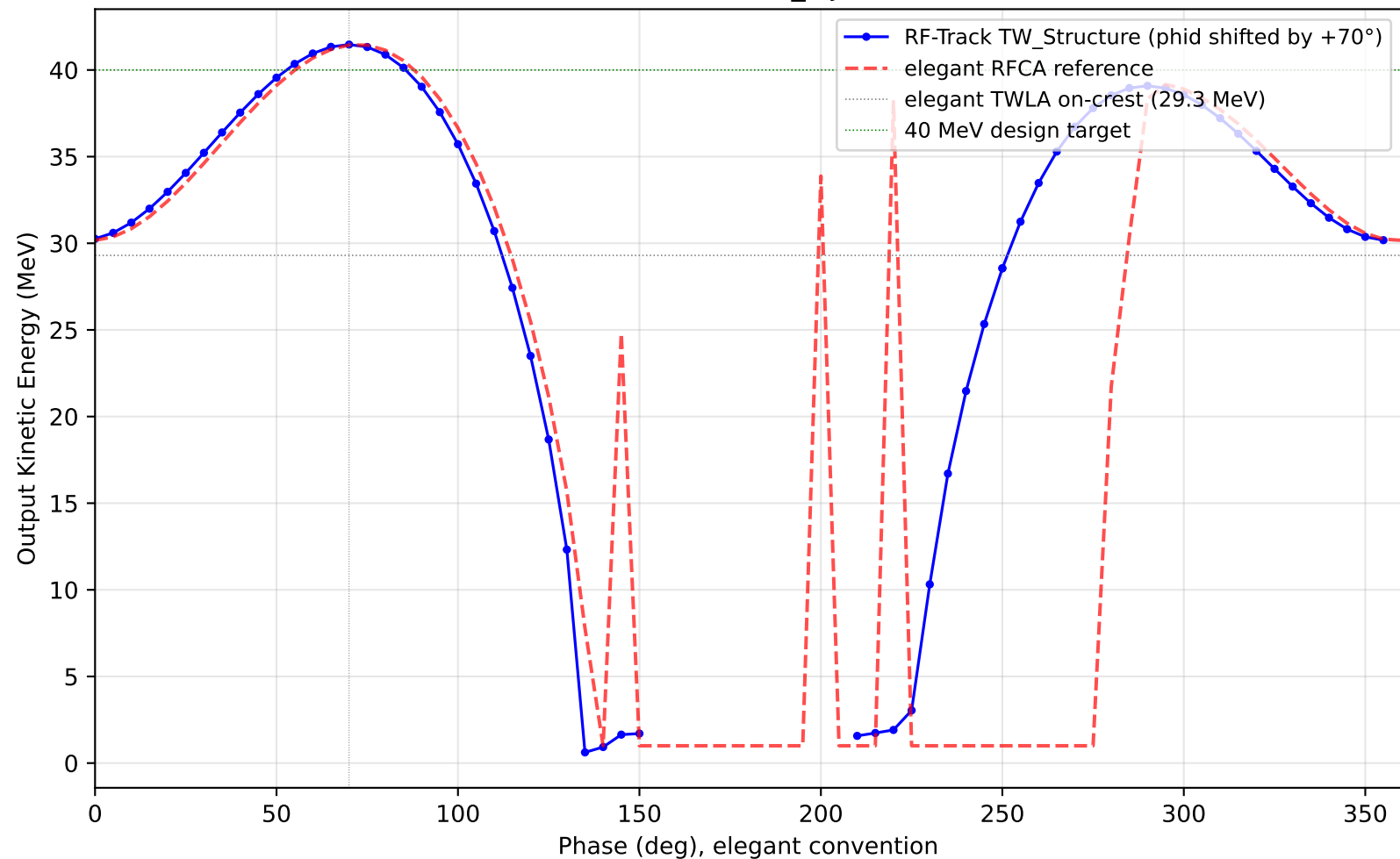
SLAC 3-m TW Linac: RF-Track vs elegant Phase Scan f=2.856 GHz, E_0=13.3 MV/m, K_{inj}=1.0 MeV, L=3.048 m
