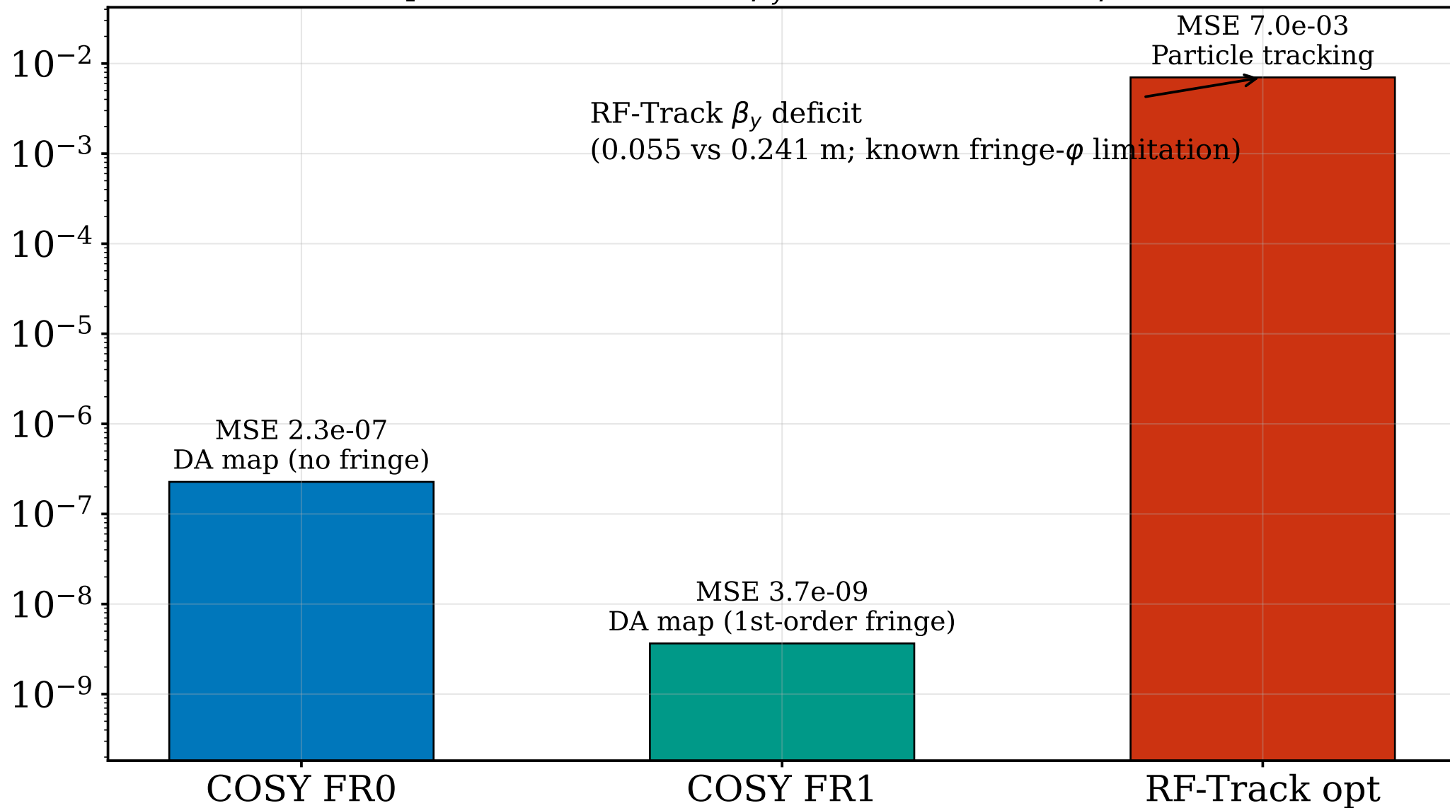
Twiss-match MSE at the undulator
