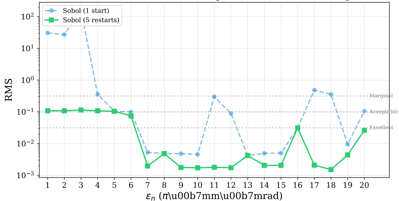
P13: Sobol Beam — Emittance Sweep (deterministic, seed-independent)
