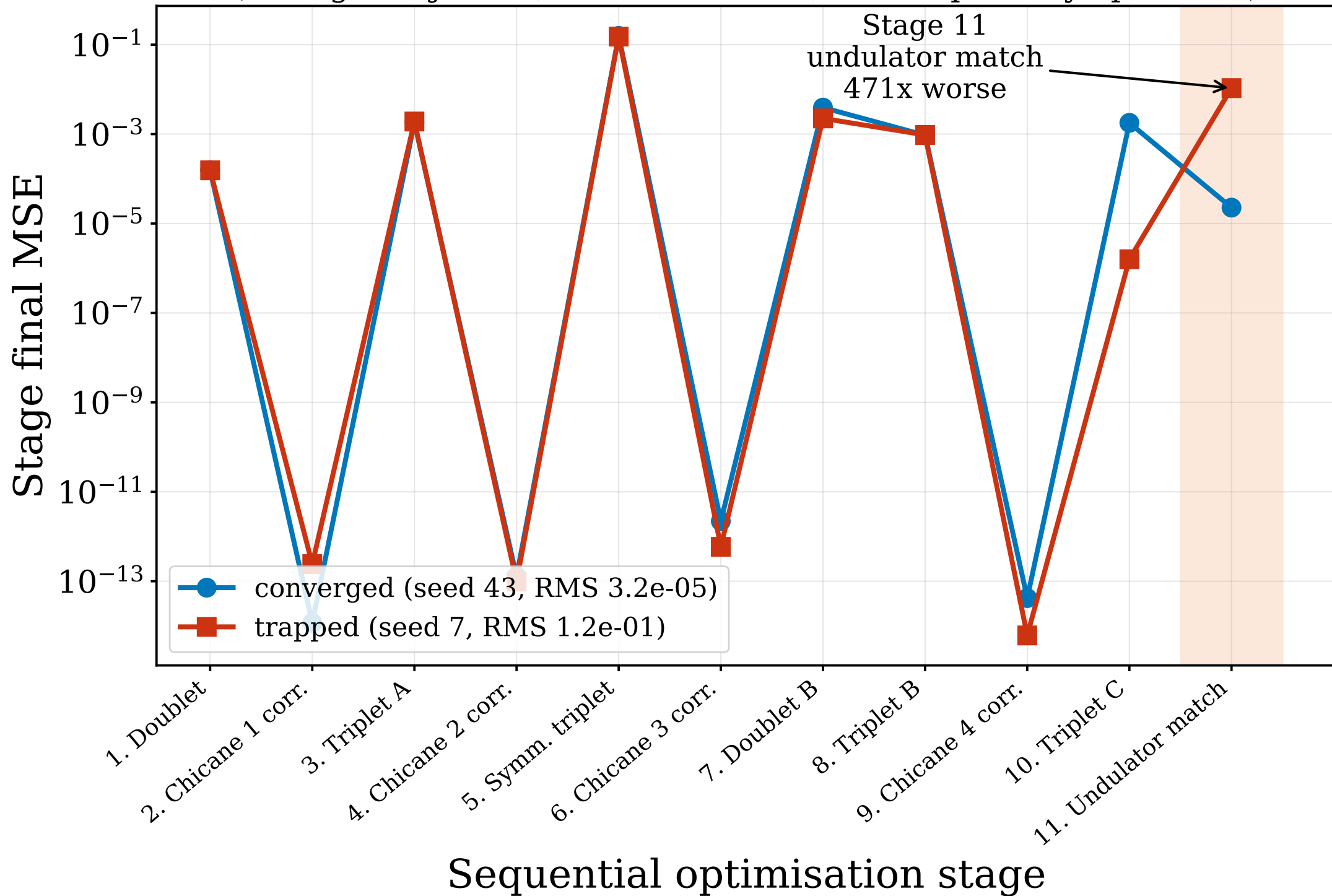
The sequential chain breaks at the final undulator match (Config A objective, two beam seeds, each separately optimised)
