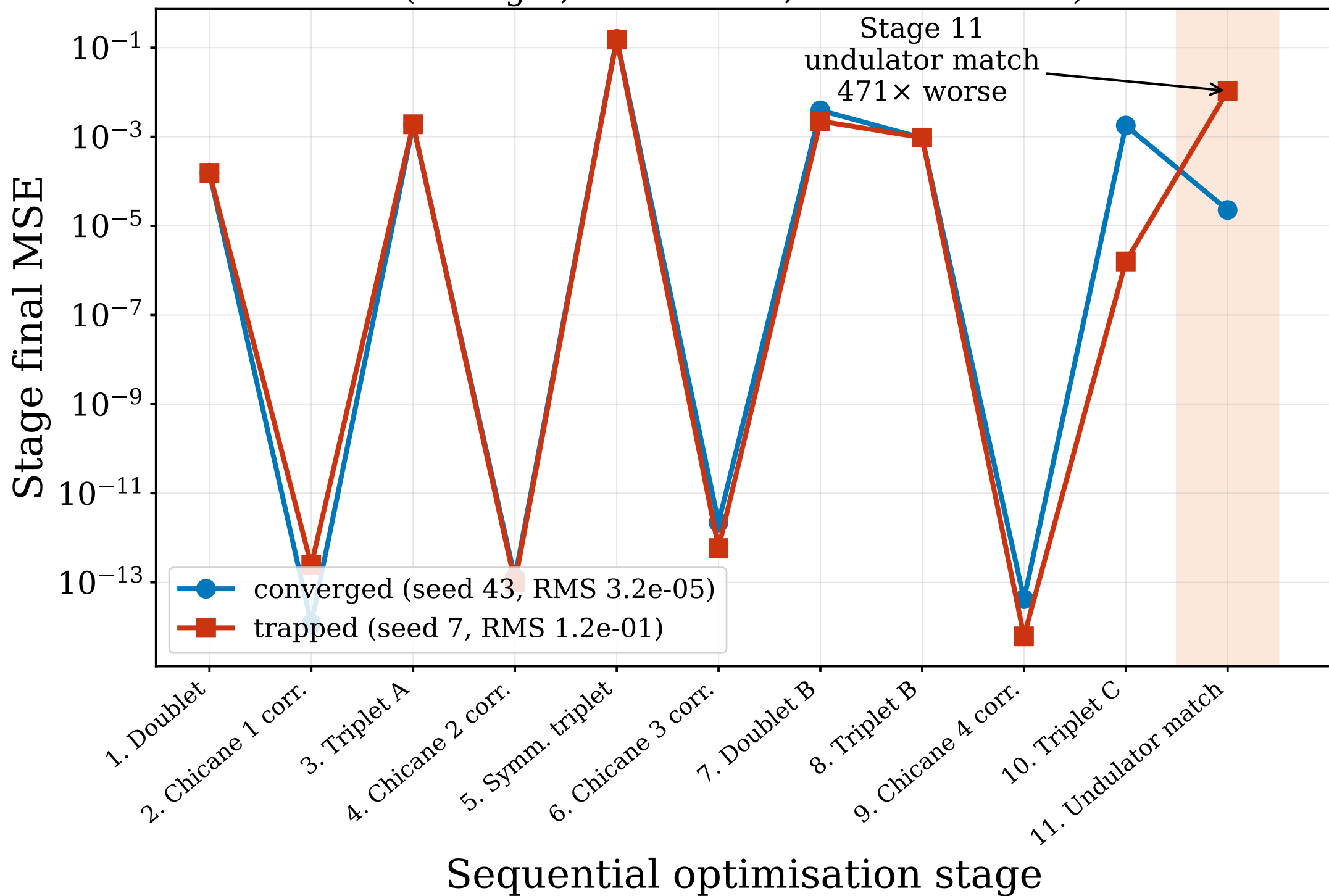
The sequential chain breaks at the final undulator match (Config A, same lattice, two beam seeds)
