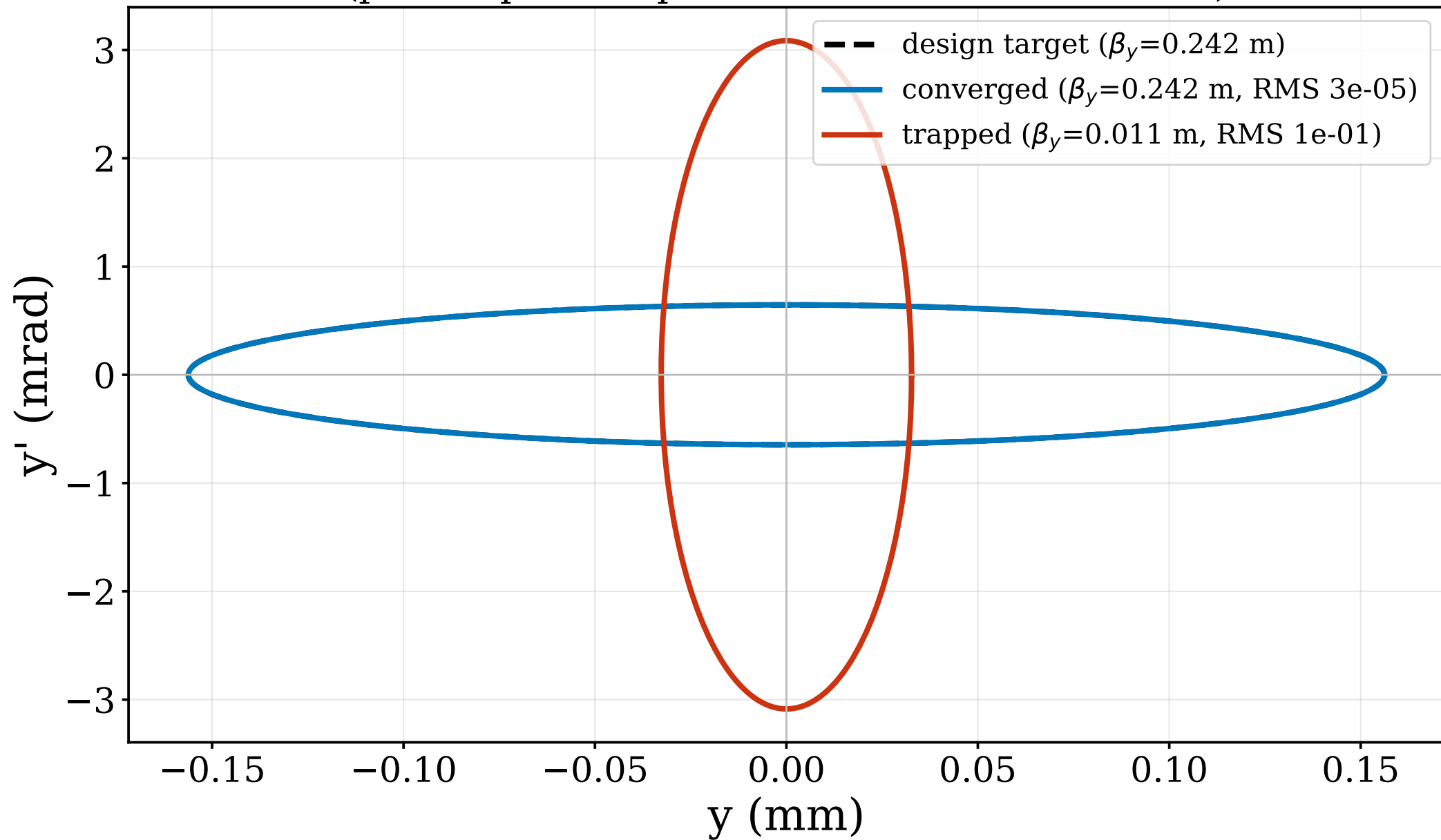
A trapped seed collapses the vertical match (phase-space ellipse at the undulator entrance)
