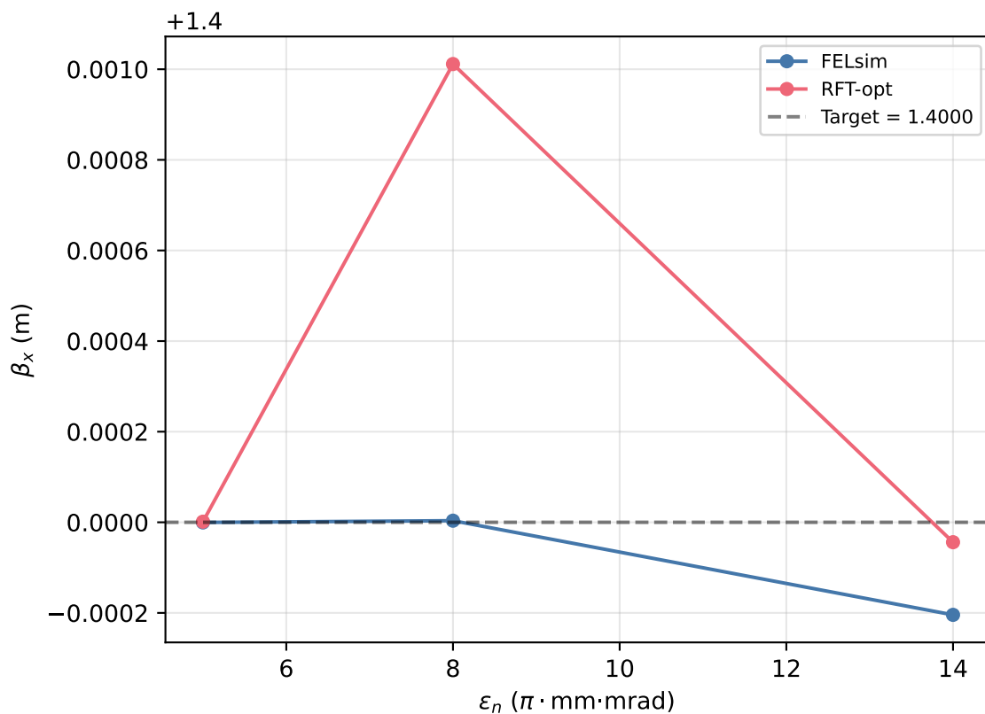
Twiss at Undulator Entrance: FELsim vs RF-Track
