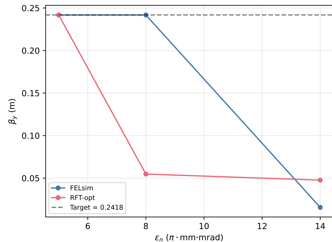
Twiss at Undulator Entrance: FELsim vs RF-Track
