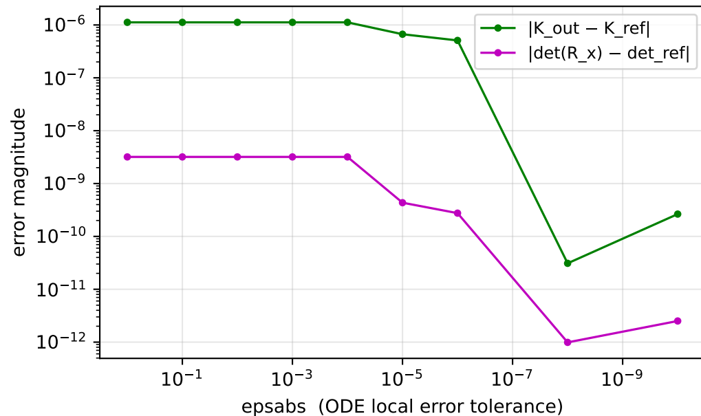
Convergence vs epsabs (nsteps = default)
