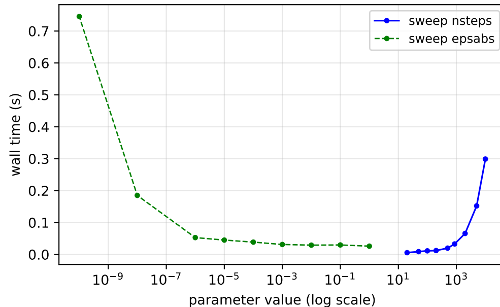
Cost of the sweeps
