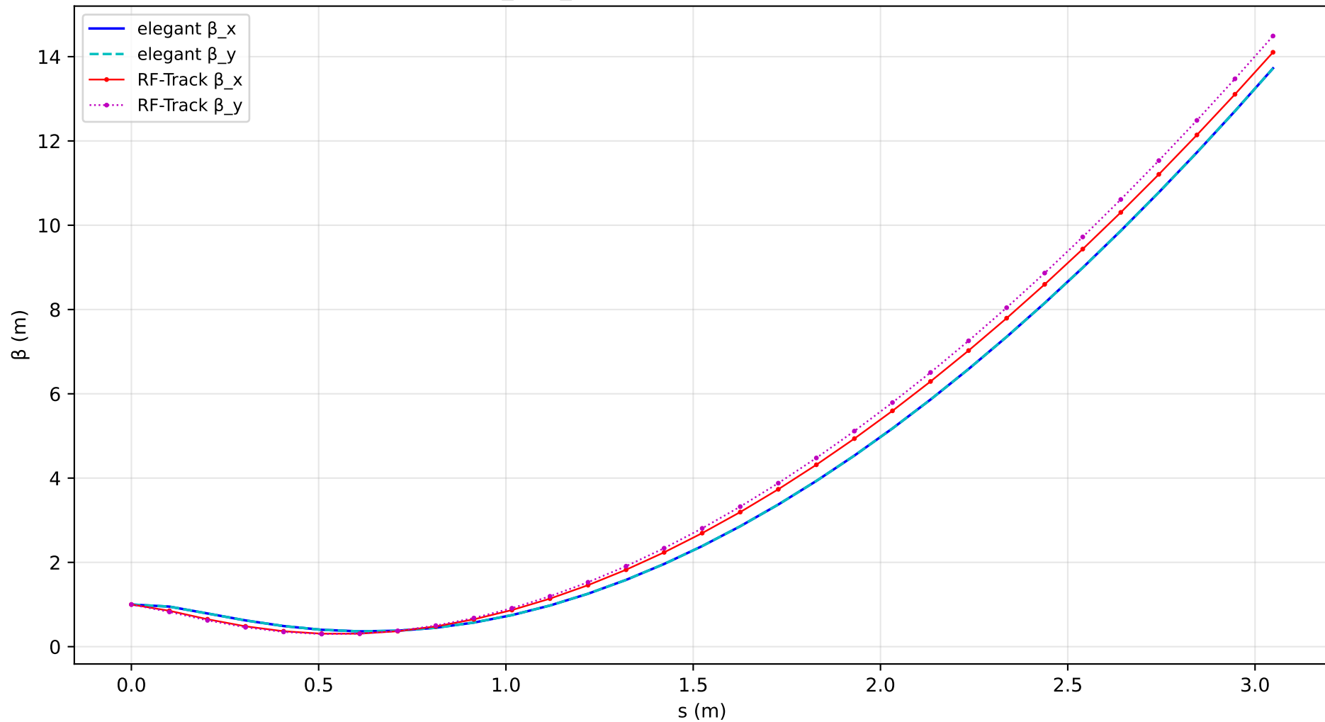
Twiss \beta Evolution Through SLAC 3-m Linac (initial \beta_x=\beta_y=1 m, \alpha=0 , on-crest/optimal phase)
