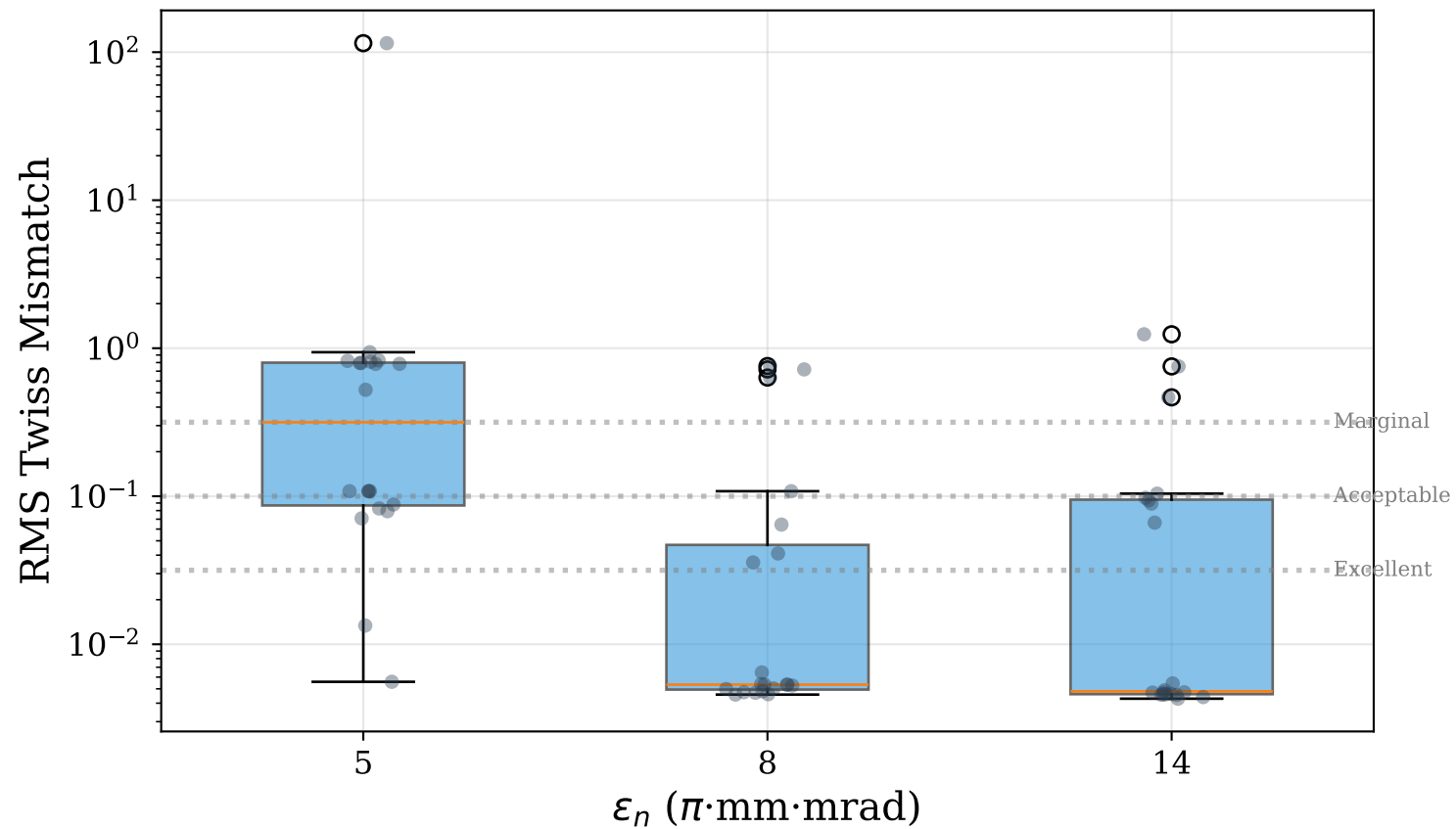
P12: RMS Distribution Across Random Seeds
