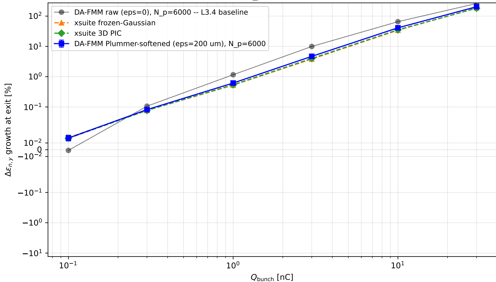
L3.7 P2: Plummer-softened DA-FMM at N_p=6000 matches xsuite across the full Q sweep
