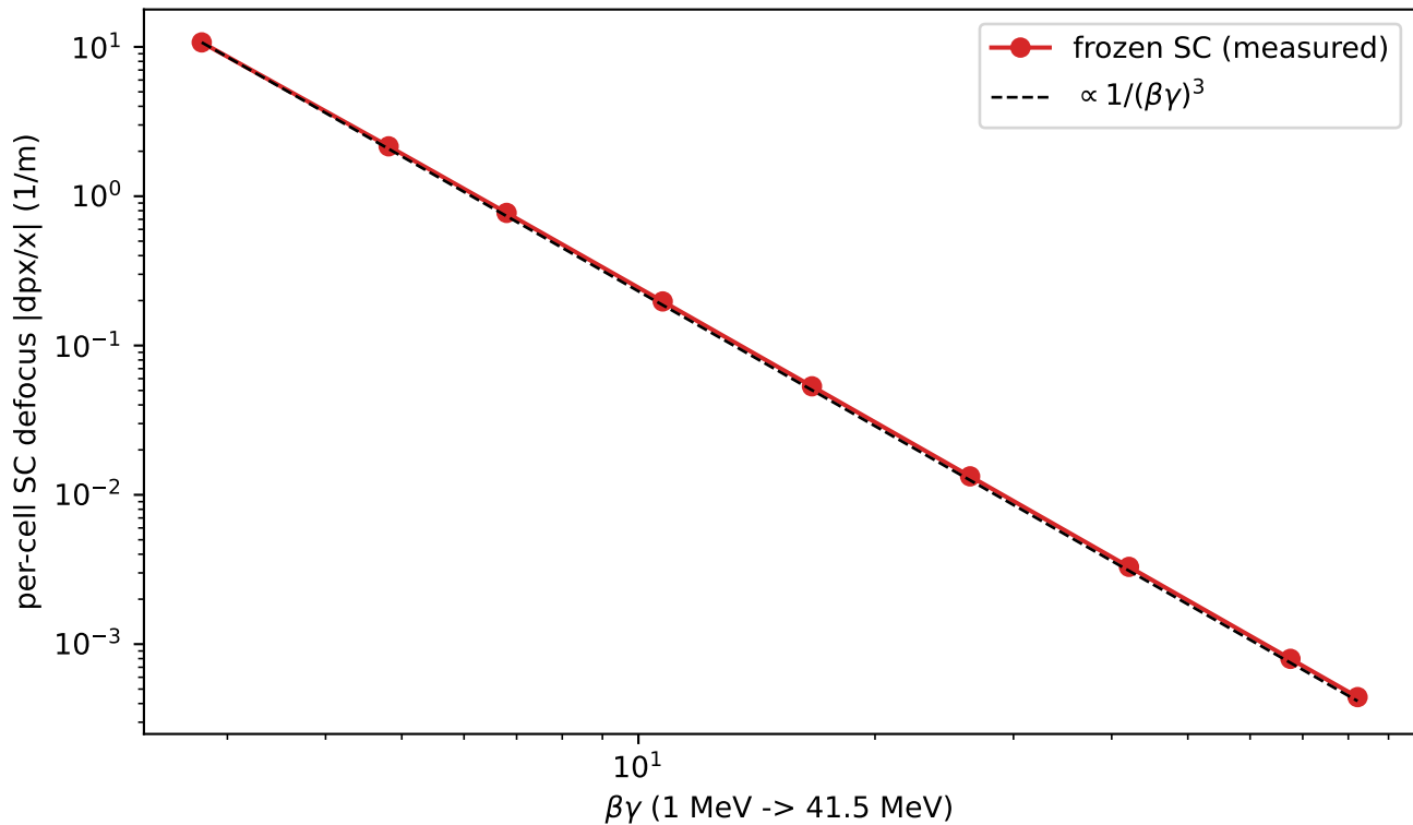
Per-cell SC follows the local energy (1/(\beta\gamma)^3)
