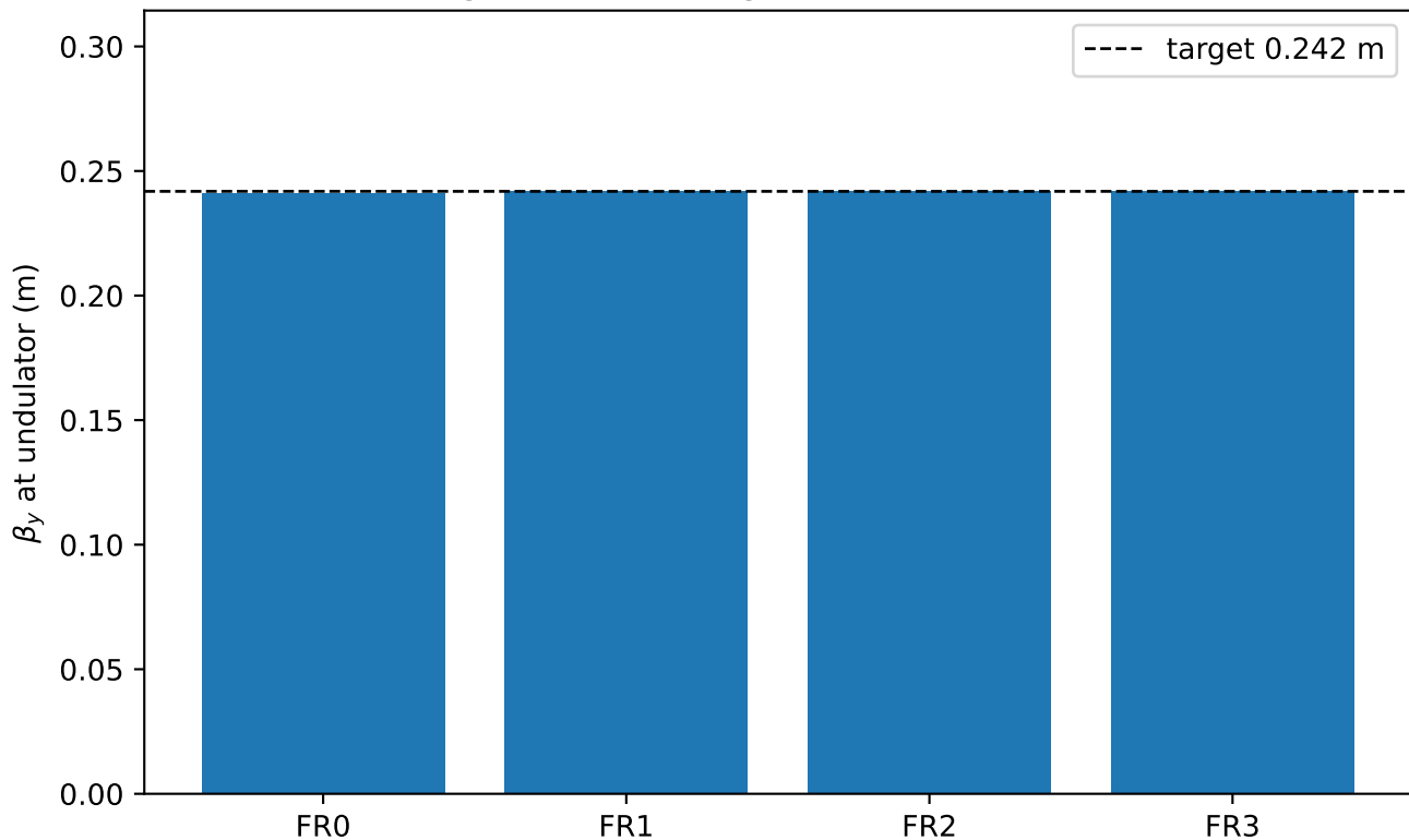
COSY fringe-order convergence to the undulator match
