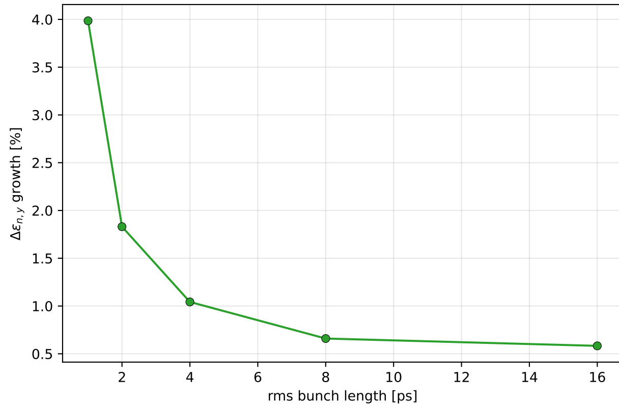
(g) Bunch-length sensitivity (45 MeV, 1 nC)
