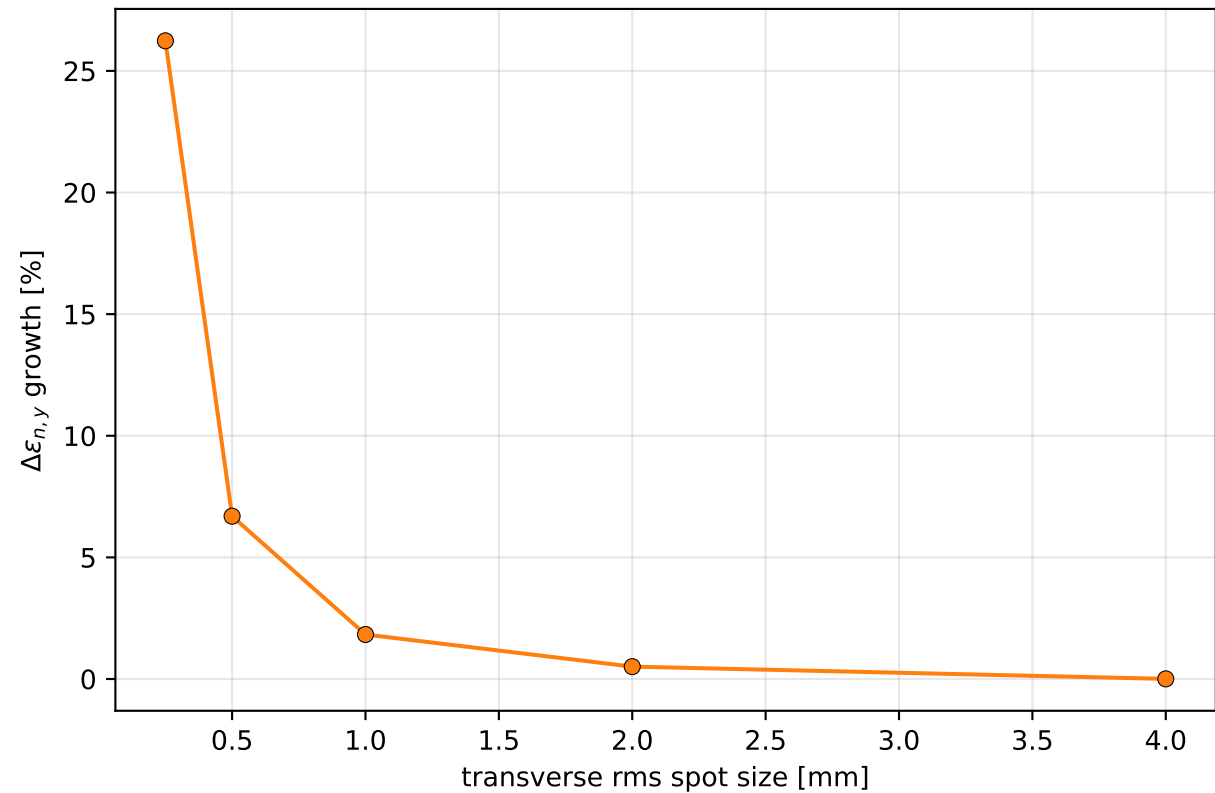
(h) Spot-size sensitivity (45 MeV, 1 nC)
