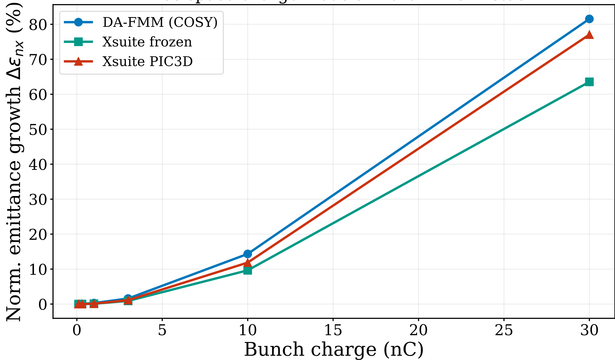
Three space-charge models in the FELsim stack
