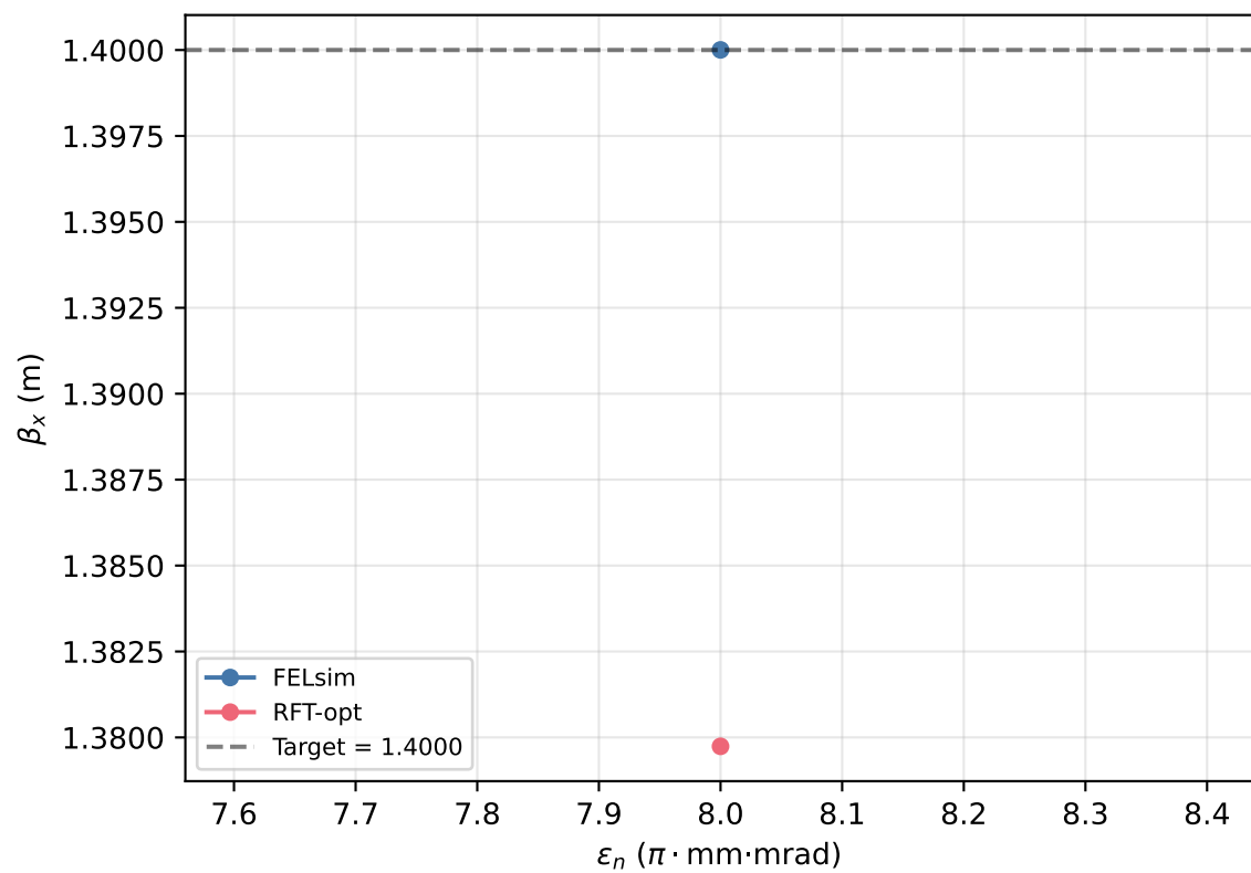
Twiss at Undulator Entrance: FELsim vs RF-Track
