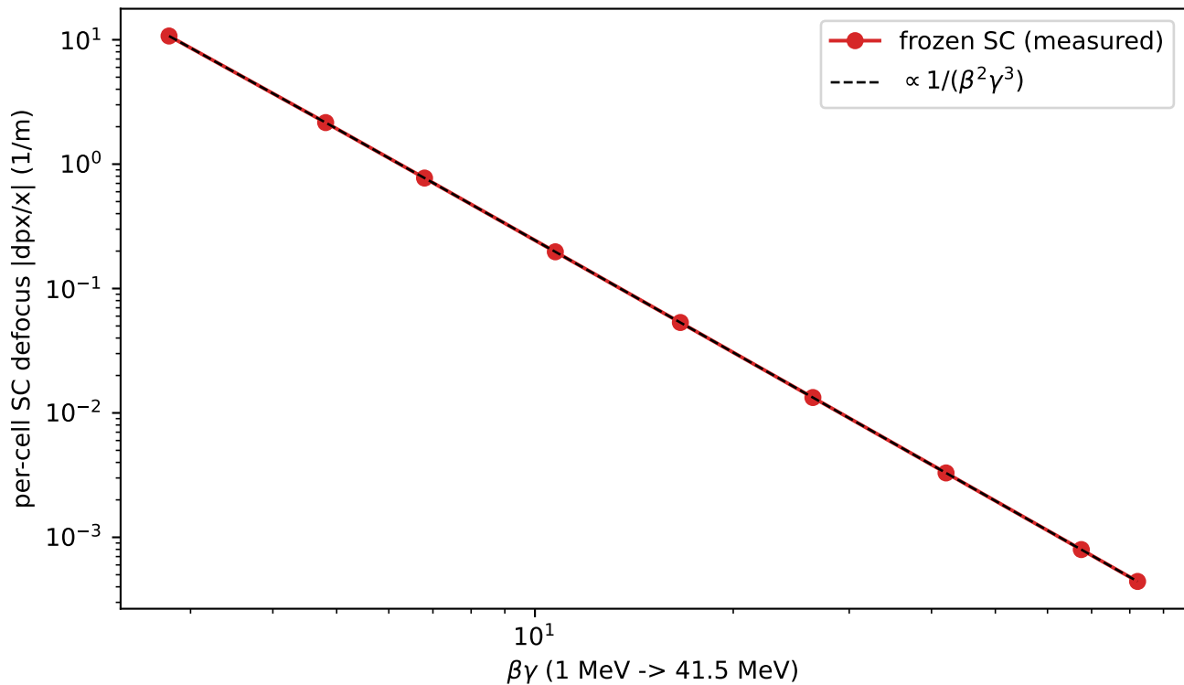
Per-cell SC follows the local energy ( \propto 1/(\beta^2\gamma^3) )
