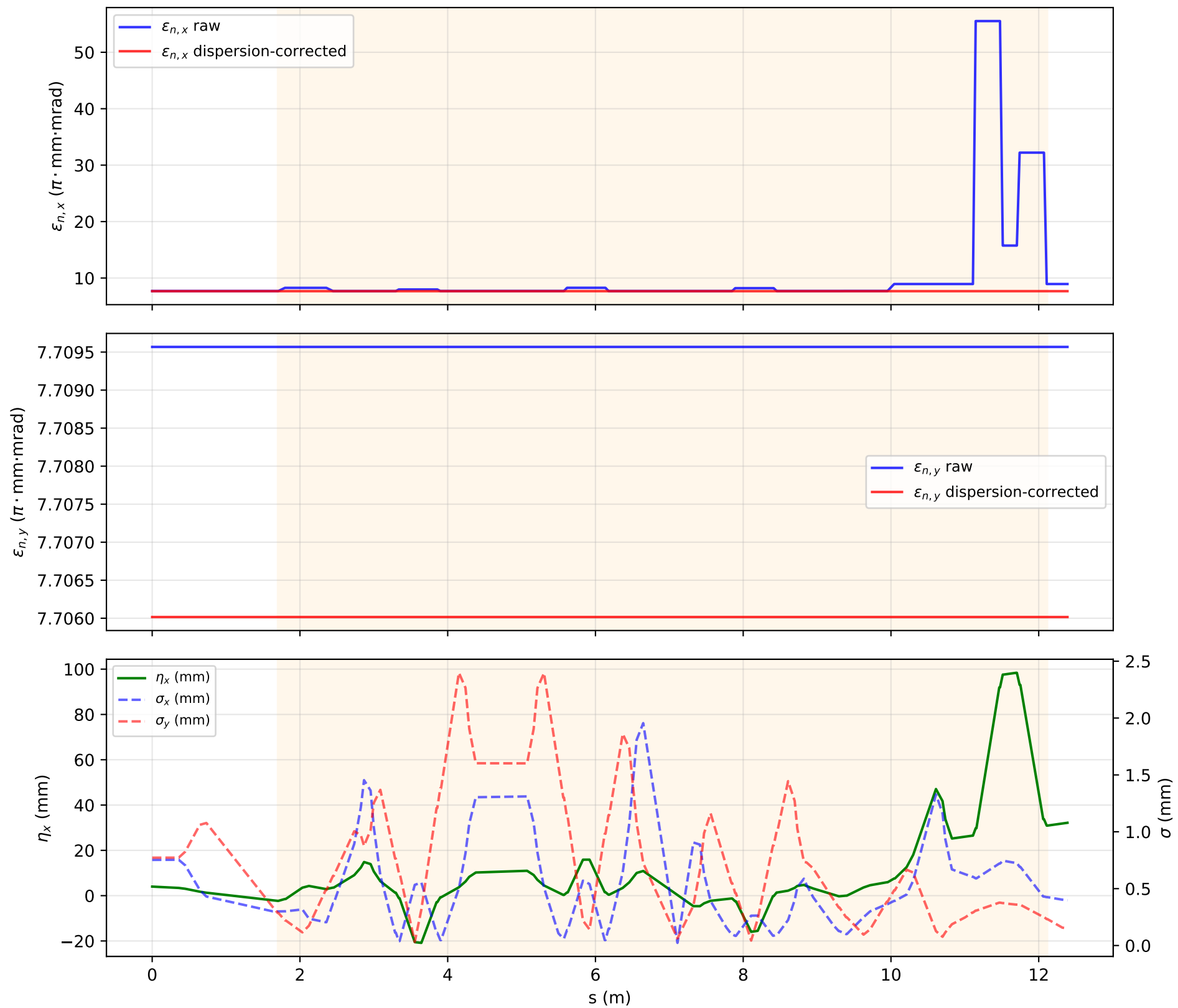
P10: Emittance Evolution Along Transport Line
