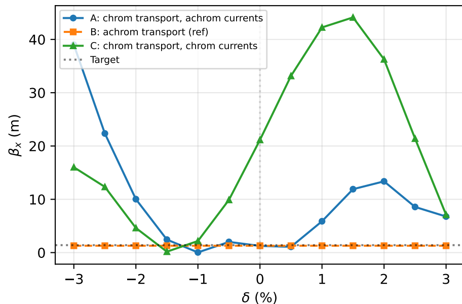
P9: Twiss Sensitivity to Energy Deviation
