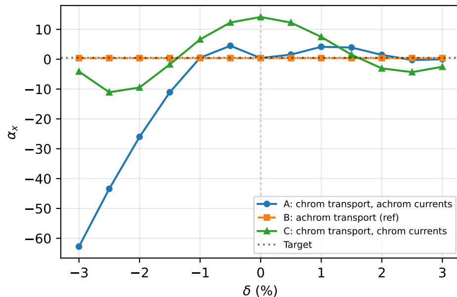
P9: Twiss Sensitivity to Energy Deviation
