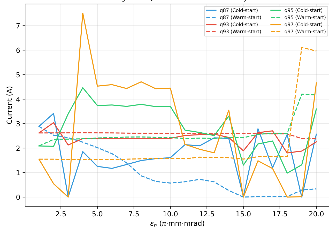
Stage 11 Quad Current Continuity
