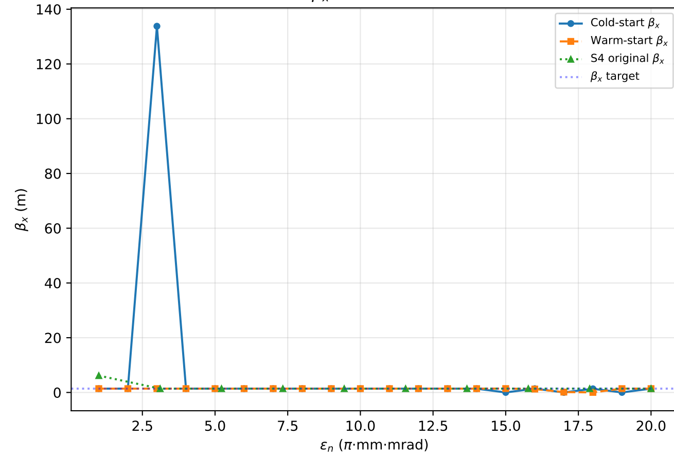
\beta_x at Undulator
