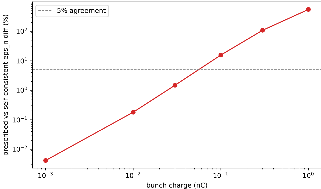
Prescribed envelope: valid for stable beams, diverges with SC
